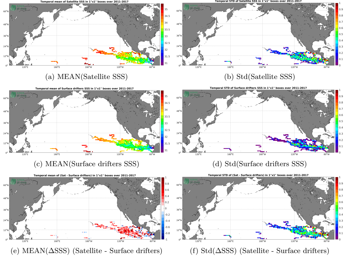
Figure 5: Temporal mean (left) and Std (right) of SSS from SMOS SSS L3 v2 - Daily - 0.5 Deg (CATDS-CECOS-IFREMER) (top), Surface drifters (middle), and of \Delta SSS (Satellite - Surface drifters). Only match-up pairs are used to generate these maps.
