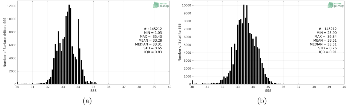
Figure 2: Histograms of SSS from Surface drifters (a) and SMOS SSS L3 v2 - Daily - 0.5 Deg (CATDS-CECOS-IFREMER) (b) considering all match-up pairs per bins of 0.1 over the North Pacific Ocean Pi-MEP region and for the full satellite product period.
