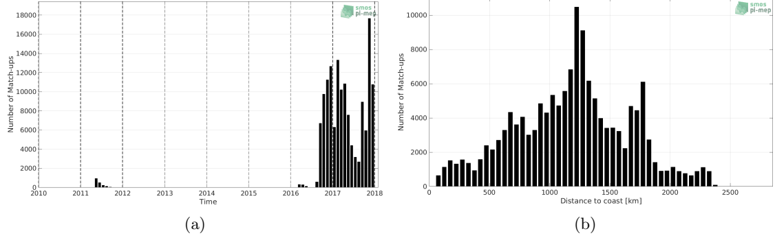
Figure 1: Number of match-ups between Surface drifters and SMOS SSS L3 v2 - Daily - 0.5 Deg (CATDS-CECOS-IFREMER) SSS as a function of time (a) and as function of the distance to coast (b) over the North Pacific Ocean Pi-MEP region and for the full satellite product period.
