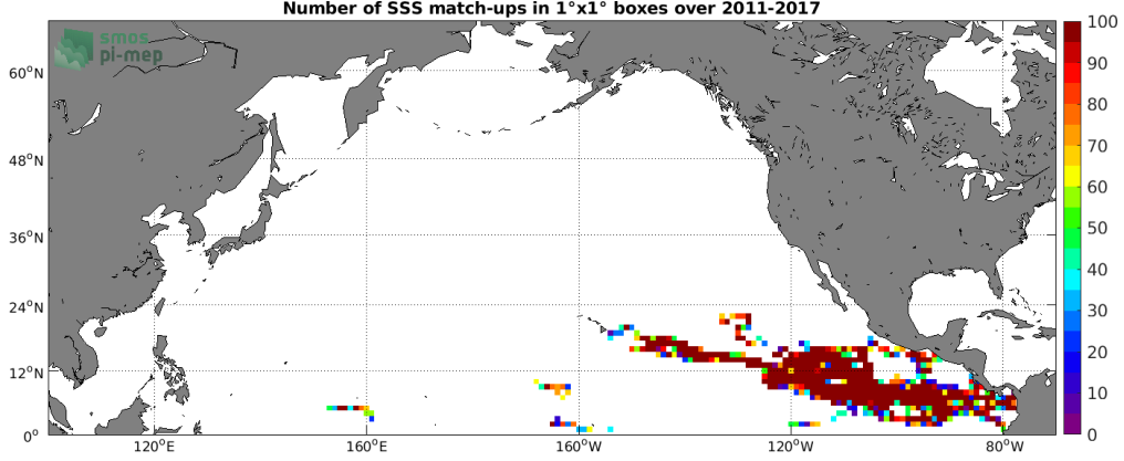
Figure 3: Number of SSS match-ups between Surface drifters SSS and the SMOS SSS L3 v2 - Daily - 0.5 Deg (CATDS-CECOS-IFREMER) SSS product for the North Pacific Ocean Pi-MEP region over 1^\circ \times 1^\circ boxes and for the full satellite product period.
