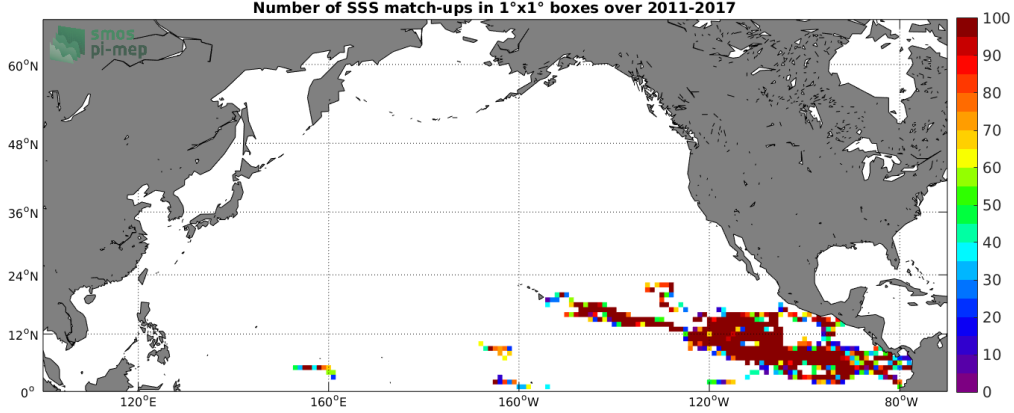
Figure 3: Number of SSS match-ups between Surface drifters SSS and the SMOS L3 v2 - Daily - 0.5 Deg (CATDS-CECOS-IFREMER) SSS product for the North Pacific Ocean Pi-MEP region over 1°x1° boxes and for the full satellite product period.
