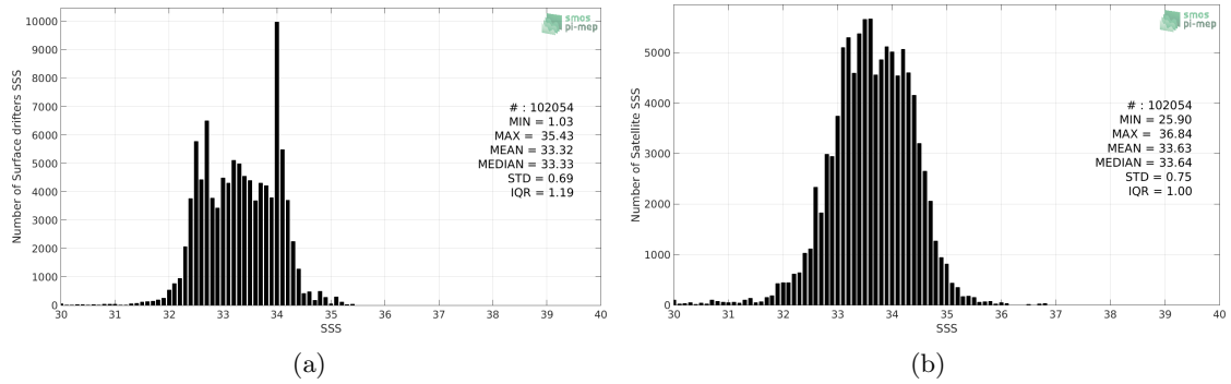
Figure 2: Histograms of SSS from Surface drifters (a) and SMOS L3 v2 - Daily - 0.5 Deg (CATDS-CECOS-IFREMER) (b) considering all match-up pairs per bins of 0.1 over the North Pacific Ocean Pi-MEP region and for the full satellite product period.
