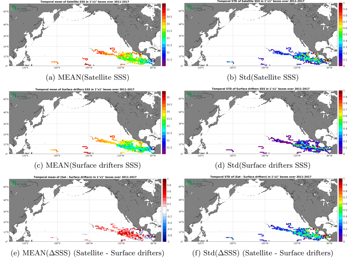
Figure 5: Temporal mean (left) and Std (right) of SSS from SMOS L3 v2 - Daily - 0.5 Deg (CATDS-CECOS-IFREMER) (top), Surface drifters (middle), and of \Delta SSS (Satellite - Surface drifters). Only match-up pairs are used to generate these maps.
