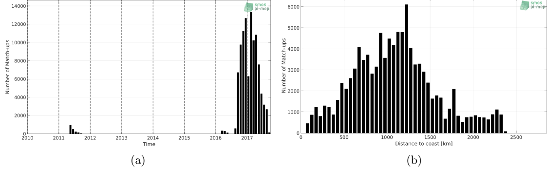
Figure 1: Number of match-ups between Surface drifters and SMOS L3 v2 - Daily - 0.5 Deg (CATDS-CECOS-IFREMER) SSS as a function of time (a) and as function of the distance to coast (b) over the North Pacific Ocean Pi-MEP region and for the full satellite product period.
