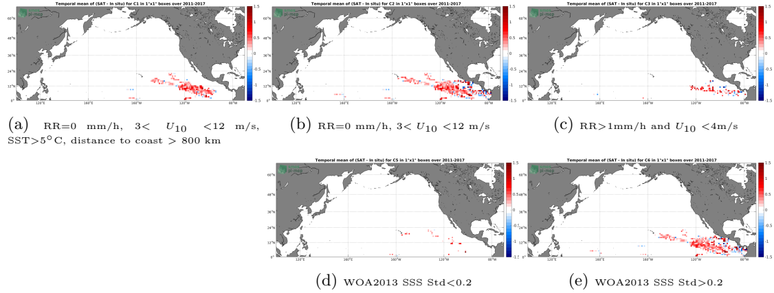
Figure 11: Temporal mean gridded over spatial boxes of size 1^{\circ}\times 1^{\circ} of \Delta\text{SSS} (SMOS L3 v2 - Daily - 0.5 Deg (CATDS-CECOS-IFREMER) - Surface drifters) for 5 different subdatasets corresponding to: RR=0 mm/h, 3 < U_{10} < 12 m/s, SST > 5^{\circ}\text{C} , distance to coast > 800 km (a), RR=0 mm/h, 3 < U_{10} < 12 m/s (b), RR > 1 mm/h and U_{10} < 4 m/s (c), WOA2013 SSS Std < 0.2 (d), WOA2013 SSS Std > 0.2 (e).
