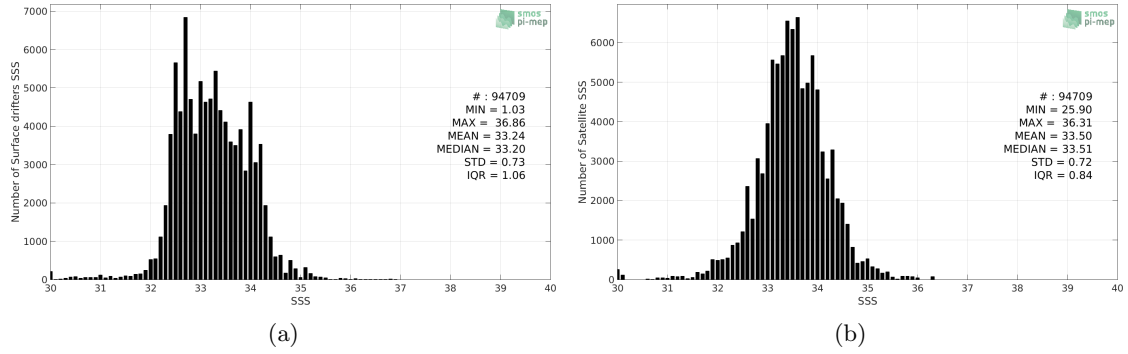
Figure 2: Histograms of SSS from Surface drifters (a) and SMOS-L3-CATDS-CECOS-IFREMER-V2-1DAY-0.5DEG (b) considering all match-up pairs per bins of 0.1 over the North Pacific Ocean Pi-MEP region and for the full satellite product period.
