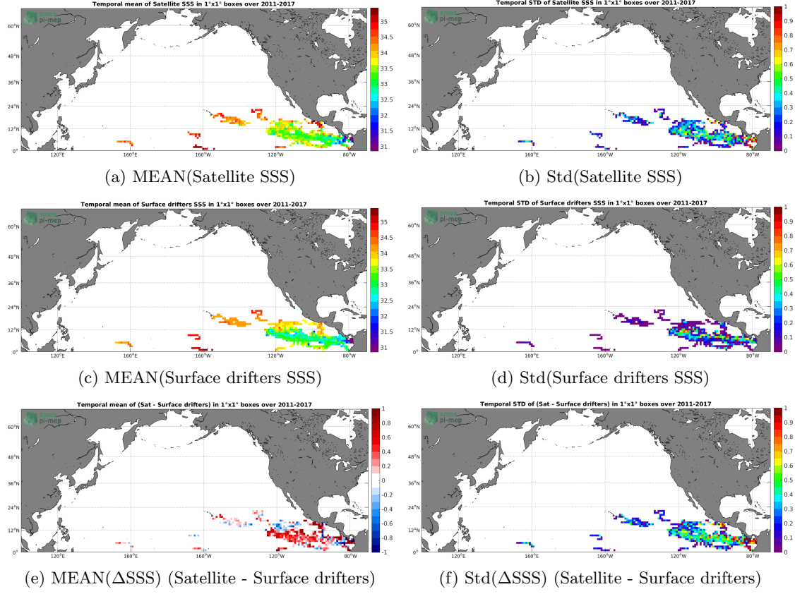
Figure 5: Temporal mean (left) and Std (right) of SSS from SMOS-L3-CATDS-CECOS-IFREMER-V2-1DAY-0.5DEG (top), Surface drifters (middle), and of \Delta SSS (Satellite - Surface drifters). Only match-up pairs are used to generate these maps.
