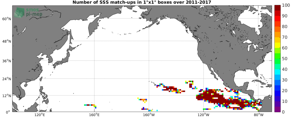
Figure 3: Number of SSS match-ups between Surface drifters SSS and the SMOS-L3-CATDS-CECOS-IFREMER-V2-1DAY-0.5DEG SSS product for the North Pacific Ocean Pi-MEP region over 1^\circ \times 1^\circ boxes and for the full satellite product period.
