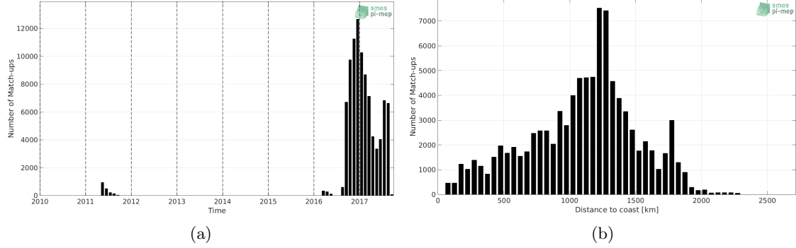
Figure 1: Number of match-ups between Surface drifters and SMOS-L3-CATDS-CECOS-IFREMER-V2-1DAY-0.5DEG SSS as a function of time (a) and as function of the distance to coast (b) over the North Pacific Ocean Pi-MEP region and for the full satellite product period.
