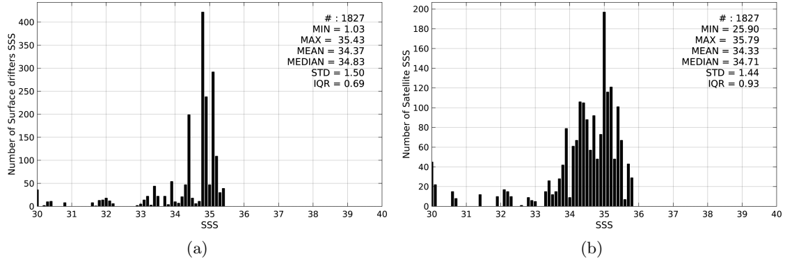
Figure 2: Histograms of SSS from Surface drifters (a) and SMOS-L3-CATDS-CECOS-IFREMER-V2-1DAY-0.5deg (b) considering all match-up pairs per bins of 0.1 over the North Pacific Ocean Pi-MEP region and for the full satellite product period.
