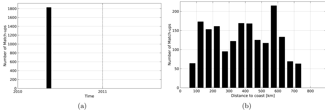
Figure 1: Number of match-ups between Surface drifters and SMOS-L3-CATDS-CECOS-IFREMER-V2-1DAY-0.5deg SSS as a function of time (a) and as function of the distance to coast (b) over the North Pacific Ocean Pi-MEP region and for the full satellite product period.
