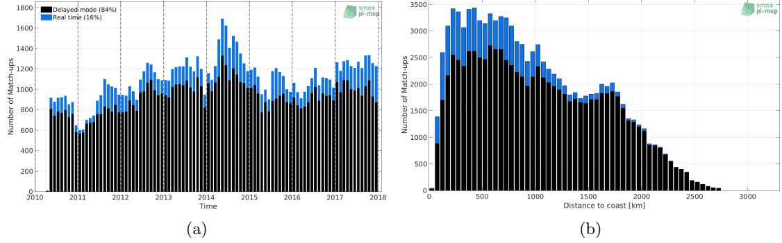
Figure 1: Number of match-ups between Argo and SMOS SSS L3 v2 - Daily - 0.5 Deg (CATDS-CECOS-IFREMER) SSS as a function of time (a) and as function of the distance to coast (b) over the North Pacific Ocean Pi-MEP region and for the full satellite product period.
