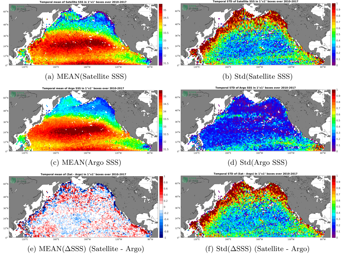
Figure 6: Temporal mean (left) and Std (right) of SSS from SMOS SSS L3 v2 - Daily - 0.5 Deg (CATDS-CECOS-IFREMER) (top), Argo (middle), and of \Delta SSS (Satellite - Argo). Only match-up pairs are used to generate these maps.
