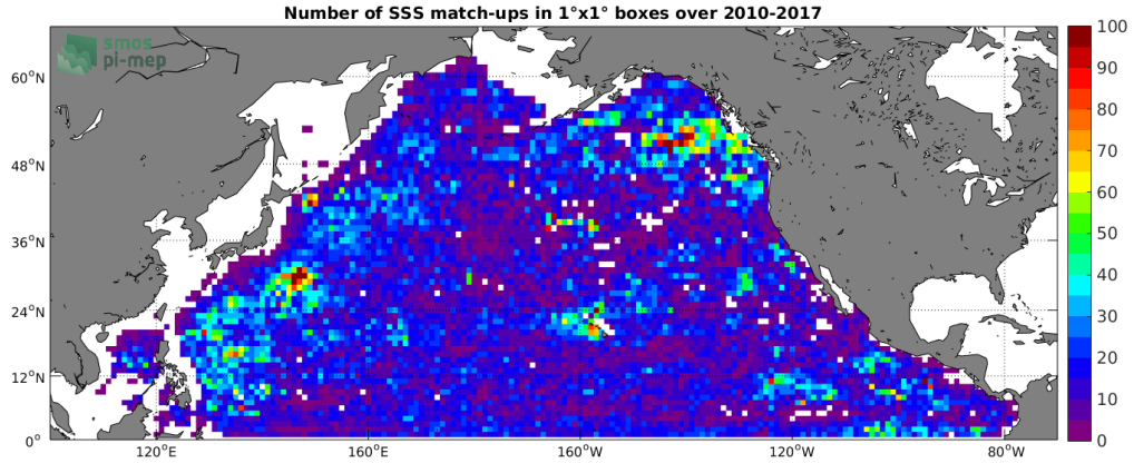
Figure 4: Number of SSS match-ups between Argo SSS and the SMOS SSS L3 v2 - Daily - 0.5 Deg (CATDS-CECOS-IFREMER) SSS product for the North Pacific Ocean Pi-MEP region over 1^\circ \times 1^\circ boxes and for the full satellite product period.
