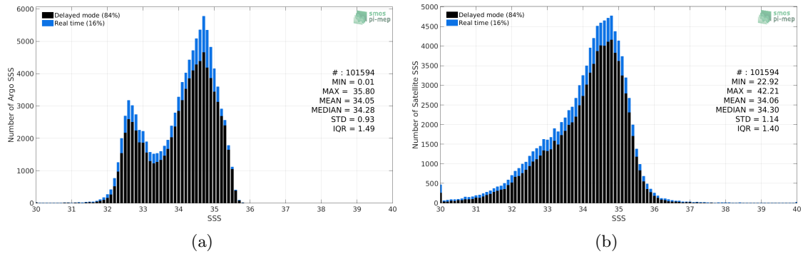
Figure 2: Histograms of SSS from Argo (a) and SMOS SSS L3 v2 - Daily - 0.5 Deg (CATDS-CECOS-IFREMER) (b) considering all match-up pairs per bins of 0.1 over the North Pacific Ocean Pi-MEP region and for the full satellite product period.
