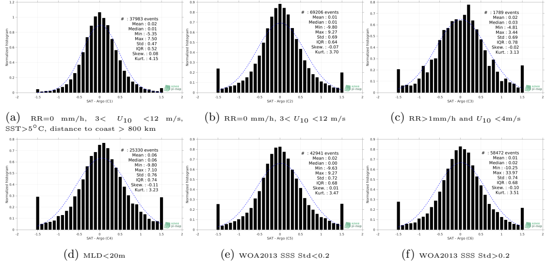
Figure 13: Normalized histogram of \Delta SSS (SMOS SSS L3 v2 - Daily - 0.5 Deg (CATDS-CECOS-IFREMER) - Argo) for 6 different subdatasets corresponding to: RR=0 mm/h, 3 < U_{10} < 12 m/s, SST>5°C, distance to coast > 800 km (a), RR=0 mm/h, 3 < U_{10} < 12 m/s (b), RR>1mm/h and U_{10} < 4 m/s (c), MLD<20m (d), WOA2013 SSS Std<0.2 (e), WOA2013 SSS Std>0.2 (f).
