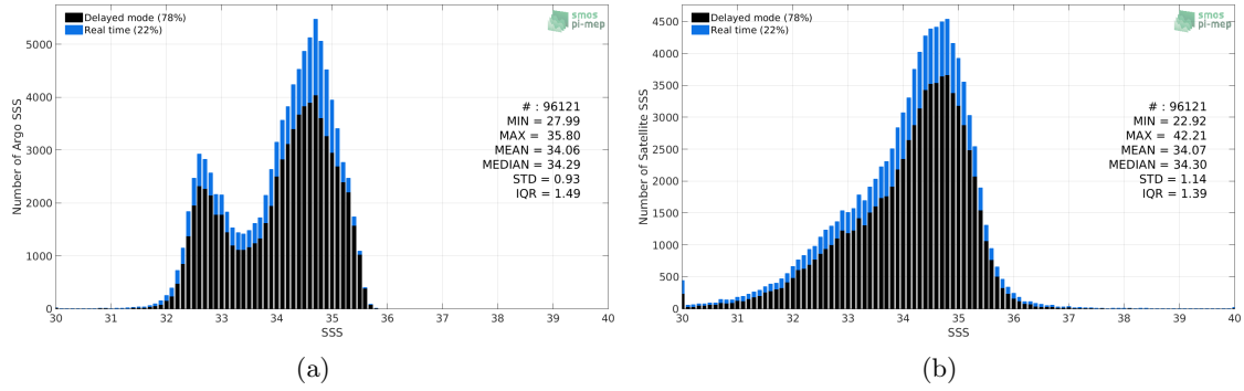
Figure 2: Histograms of SSS from Argo (a) and SMOS L3 v2 - Daily - 0.5 Deg (CATDS-CECOS-IFREMER) (b) considering all match-up pairs per bins of 0.1 over the North Pacific Ocean Pi-MEP region and for the full satellite product period.
