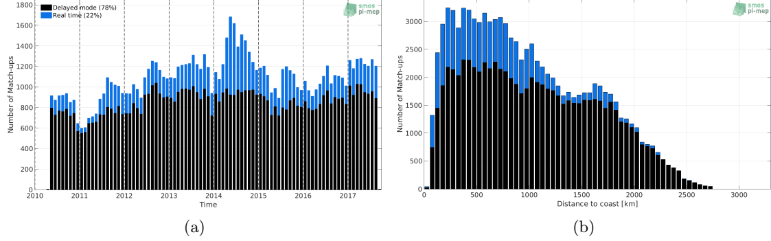
Figure 1: Number of match-ups between Argo and SMOS L3 v2 - Daily - 0.5 Deg (CATDS-CECOS-IFREMER) SSS as a function of time (a) and as function of the distance to coast (b) over the North Pacific Ocean Pi-MEP region and for the full satellite product period.
