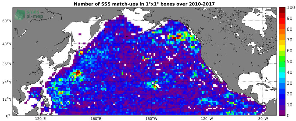
Figure 4: Number of SSS match-ups between Argo SSS and the SMOS L3 v2 - Daily - 0.5 Deg (CATDS-CECOS-IFREMER) SSS product for the North Pacific Ocean Pi-MEP region over 1^\circ \times 1^\circ boxes and for the full satellite product period.
