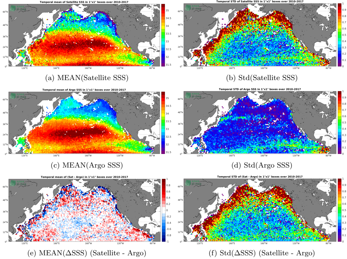
Figure 6: Temporal mean (left) and Std (right) of SSS from SMOS L3 v2 - Daily - 0.5 Deg (CATDS-CECOS-IFREMER) (top), Argo (middle), and of \Delta SSS (Satellite - Argo). Only match-up pairs are used to generate these maps.
