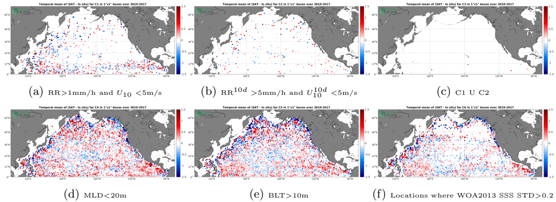
Figure 12: Temporal mean gridded over spatial boxes of size 1°x1° of \Delta SSS (SMOS-L3-CATDS-CECOS-IFREMER-V2-1DAY-0.5DEG - Argo) for 6 different subdatasets corresponding to:RR>1mm/h and U_{10} < 5m/s (a), RR^{10d} > 5mm/h and U_{10}^{10d} < 5m/s (b), C1 U C2 (c),MLD<20m (d),BLT>10m (e),Locations where WOA2013 SSS STD>0.2 (f).
