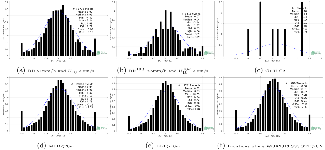
Figure 13: Normalized histogram of \Delta\text{SSS} (SMOS-L3-CATDS-CECOS-IFREMER-V2-1DAY-0.5DEG - Argo) for 6 different subdatasets corresponding to: \text{RR}>1\text{mm/h} and U_{10}<5\text{m/s} (a), \text{RR}^{10d}>5\text{mm/h} and U_{10}^{10d}<5\text{m/s} (b), C1 U C2 (c), \text{MLD}<20\text{m} (d), \text{BLT}>10\text{m} (e), Locations where WOA2013 SSS STD >0.2 (f).
