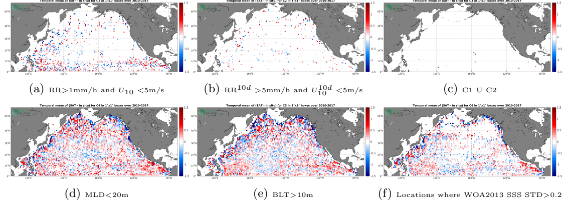
Figure 12: Temporal mean gridded over spatial boxes of size 1^\circ \times 1^\circ of \Delta\text{SSS} (SMOS-L3-CATDS-CECOS-IFREMER-V2-1DAY-0.5DEG - Argo) for 6 different subdatasets corresponding to: \text{RR}>1\text{mm/h} and U_{10}<5\text{m/s} (a), \text{RR}^{10d}>5\text{mm/h} and U_{10}^{10d}<5\text{m/s} (b), C1 U C2 (c), \text{MLD}<20\text{m} (d), \text{BLT}>10\text{m} (e), Locations where WOA2013 SSS STD >0.2 (f).
