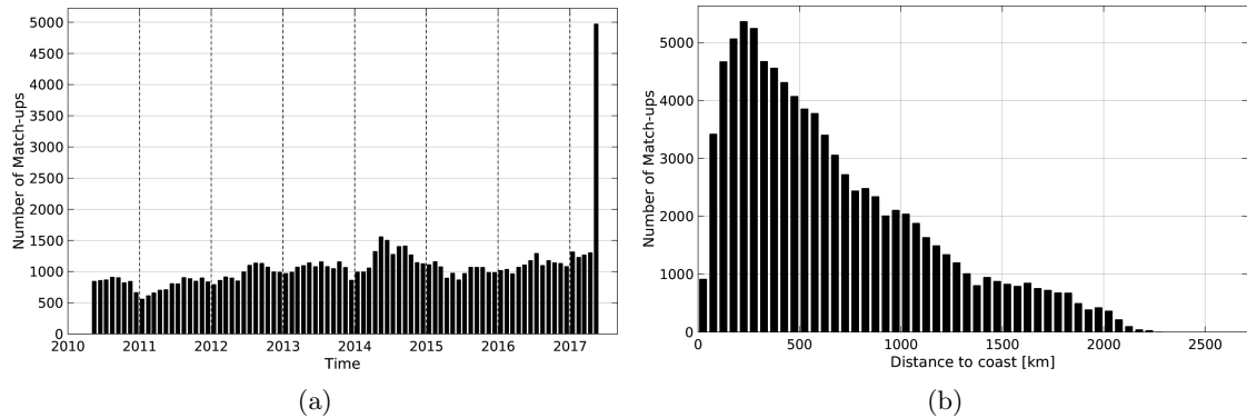
Figure 1: Number of match-ups between Argo and SMOS-L3-CATDS-CECOS-IFREMER-V2-1DAY-0.5deg SSS as a function of time (a) and as function of the distance to coast (b) over the North Pacific Ocean Pi-MEP region and for the full satellite product period.
