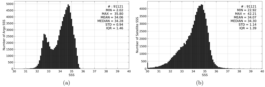
Figure 2: Histograms of SSS from Argo (a) and SMOS-L3-CATDS-CECOS-IFREMER-V2-1DAY-0.5deg (b) considering all match-up pairs per bins of 0.1 over the North Pacific Ocean Pi-MEP region and for the full satellite product period.
