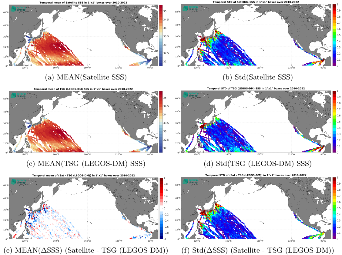
Figure 7: Temporal mean (left) and Std (right) of SSS from SMOS SSS L3 v335 - Monthly - 25 km (CATDS-CPDC) (top), TSG (LEGOS-DM) (middle), and of \Delta\text{SSS} (Satellite - TSG (LEGOS-DM)). Only match-up pairs are used to generate these maps.
