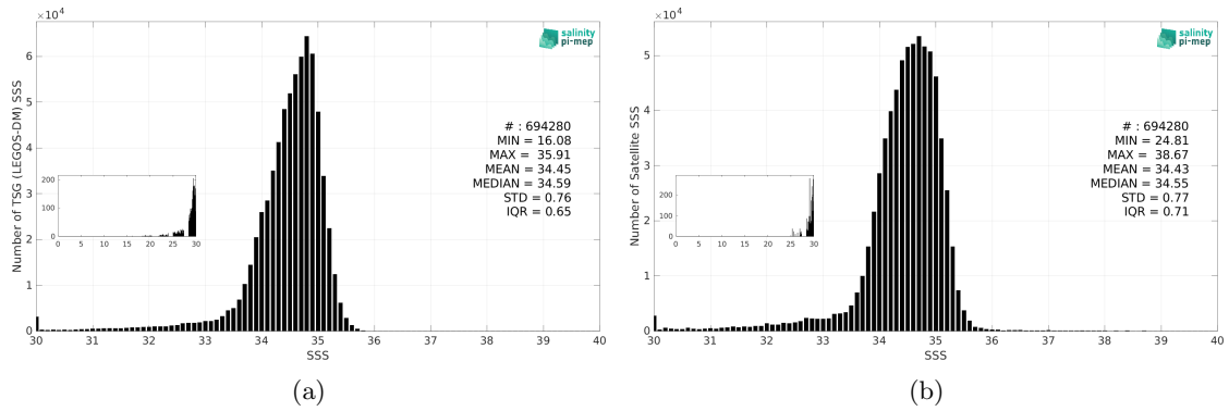
Figure 3: Histograms of SSS from TSG (LEGOS-DM) (a) and SMOS SSS L3 v335 - Monthly - 25 km (CATDS-CPDC) (b) considering all match-up pairs per bins of 0.1 over the North Pacific Ocean Pi-MEP region and for the full satellite product period.
