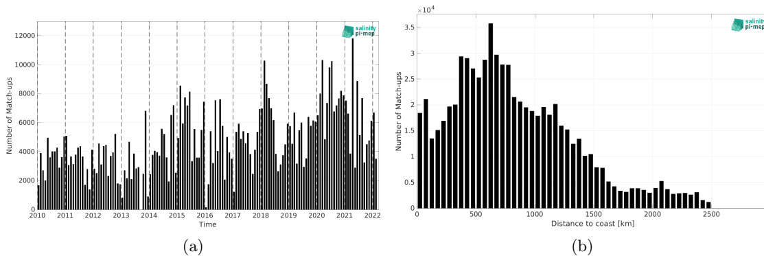
Figure 2: Number of match-ups between TSG (LEGOS-DM) and SMOS SSS L3 v335 - Monthly - 25 km (CATDS-CPDC) SSS as a function of time (a) and as function of the distance to coast (b) over the North Pacific Ocean Pi-MEP region and for the full satellite product period.
