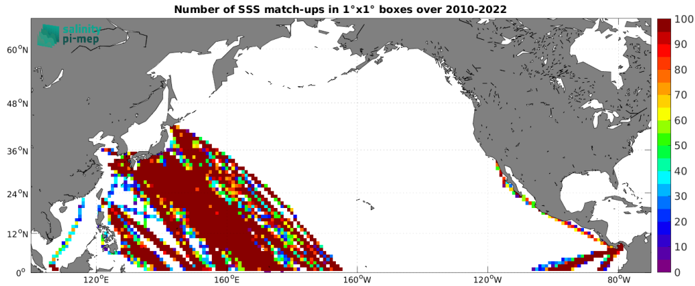
Figure 5: Number of SSS match-ups between TSG (LEGOS-DM) SSS and the SMOS SSS L3 v335 - Monthly - 25 km (CATDS-CPDC) SSS product for the North Pacific Ocean Pi-MEP region over 1^\circ \times 1^\circ boxes and for the full satellite product period.
