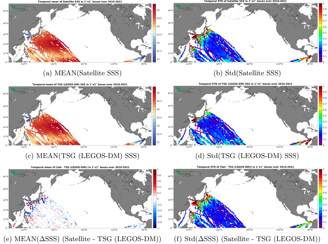
Figure 6: Temporal mean (left) and Std (right) of SSS from SMOS SSS L3 v335 - Monthly - 25 km (CATDS-CPDC) (top), TSG (LEGOS-DM) (middle), and of \Delta\text{SSS} (Satellite - TSG (LEGOS-DM)). Only match-up pairs are used to generate these maps.
