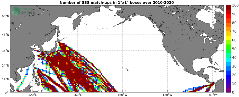
Figure 4: Number of SSS match-ups between TSG (LEGOS-DM) SSS and the SMOS SSS L3 v335 - Monthly - 25 km (CATDS-CPDC) SSS product for the North Pacific Ocean Pi-MEP region over 1^\circ \times 1^\circ boxes and for the full satellite product period.
