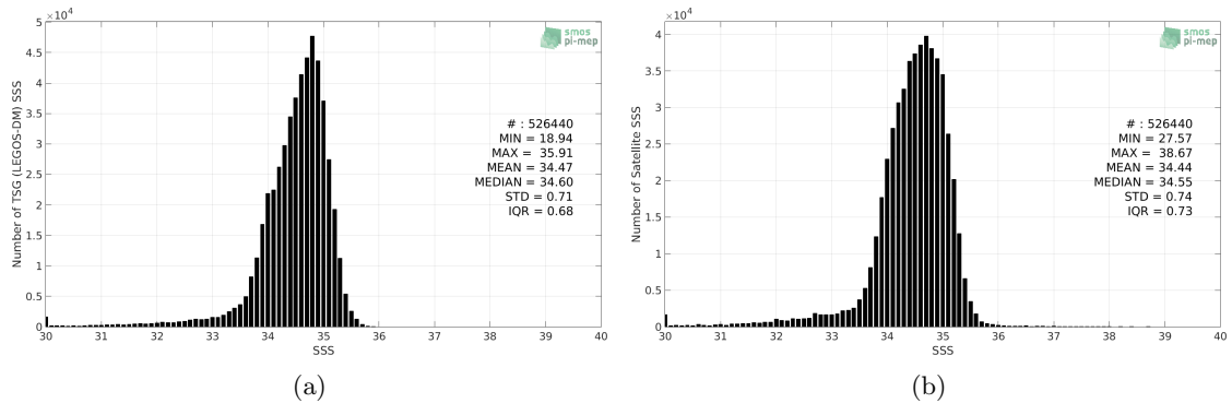
Figure 2: Histograms of SSS from TSG (LEGOS-DM) (a) and SMOS SSS L3 v335 - Monthly - 25 km (CATDS-CPDC) (b) considering all match-up pairs per bins of 0.1 over the North Pacific Ocean Pi-MEP region and for the full satellite product period.
