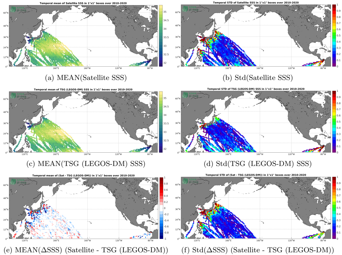
Figure 6: Temporal mean (left) and Std (right) of SSS from SMOS SSS L3 v335 - Monthly - 25 km (CATDS-CPDC) (top), TSG (LEGOS-DM) (middle), and of \Delta SSS (Satellite - TSG (LEGOS-DM)). Only match-up pairs are used to generate these maps.
