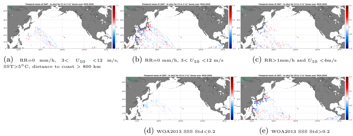
Figure 12: Temporal mean gridded over spatial boxes of size 1^\circ \times 1^\circ of \Delta SSS (SMOS SSS L3 v335 - Monthly - 25 km (CATDS-CPDC) - TSG (LEGOS-DM)) for 5 different subdatasets corresponding to:RR=0 mm/h, 3 < U_{10} < 12 m/s, SST >5^\circ\text{C} , distance to coast > 800 km (a), RR=0 mm/h, 3 < U_{10} < 12 m/s (b), RR >1 mm/h and U_{10} < 4 m/s (c), WOA2013 SSS Std <0.2 (d), WOA2013 SSS Std >0.2 (e).
