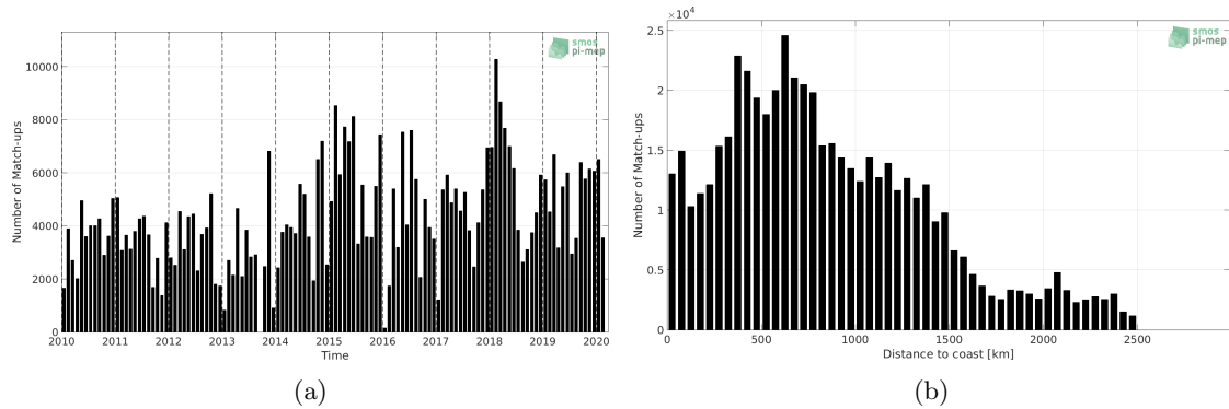
Figure 1: Number of match-ups between TSG (LEGOS-DM) and SMOS SSS L3 v335 - Monthly - 25 km (CATDS-CPDC) SSS as a function of time (a) and as function of the distance to coast (b) over the North Pacific Ocean Pi-MEP region and for the full satellite product period.
