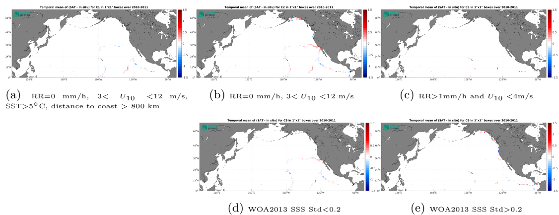
Figure 14: Temporal mean gridded over spatial boxes of size 1^\circ \times 1^\circ of \Delta SSS (SMOS SSS L3 v335 - Monthly - 25 km (CATDS-CPDC) - TSG (GOSUD-Sailing-ship)) for 5 different subdatasets corresponding to:RR=0 mm/h, 3 < U_{10} < 12 m/s, SST >5^\circ C, distance to coast > 800 km (a), RR=0 mm/h, 3 < U_{10} < 12 m/s (b), RR >1 mm/h and U_{10} < 4 m/s (c), WOA2013 SSS Std <0.2 (d), WOA2013 SSS Std >0.2 (e).
