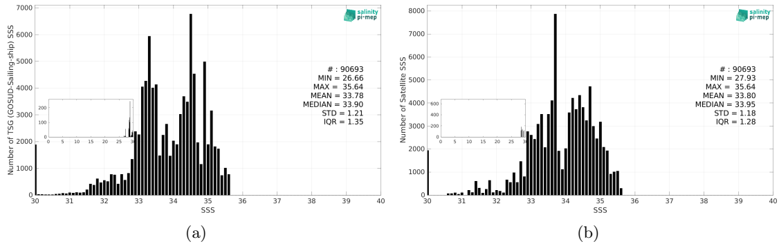
Figure 3: Histograms of SSS from TSG (GOSUD-Sailing-ship) (a) and SMOS SSS L3 v335 - Monthly - 25 km (CATDS-CPDC) (b) considering all match-up pairs per bins of 0.1 over the North Pacific Ocean Pi-MEP region and for the full satellite product period.
