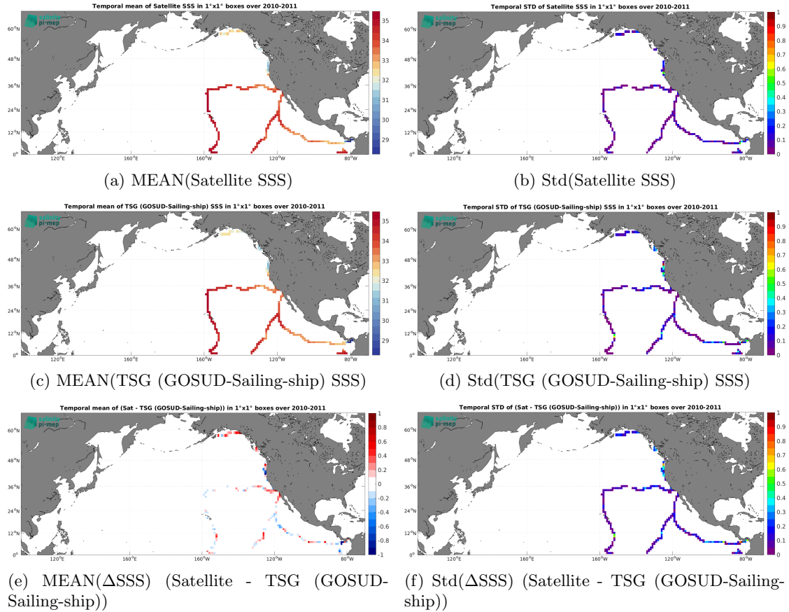
Figure 7: Temporal mean (left) and Std (right) of SSS from SMOS SSS L3 v335 - Monthly - 25 km (CATDS-CPDC) (top), TSG (GOSUD-Sailing-ship) (middle), and of \Delta SSS (Satellite - TSG (GOSUD-Sailing-ship)). Only match-up pairs are used to generate these maps.
