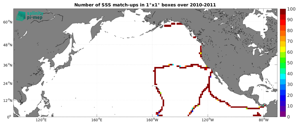
Figure 5: Number of SSS match-ups between TSG (GOSUD-Sailing-ship) SSS and the SMOS SSS L3 v335 - Monthly - 25 km (CATDS-CPDC) SSS product for the North Pacific Ocean Pi-MEP region over 1^\circ \times 1^\circ boxes and for the full satellite product period.
