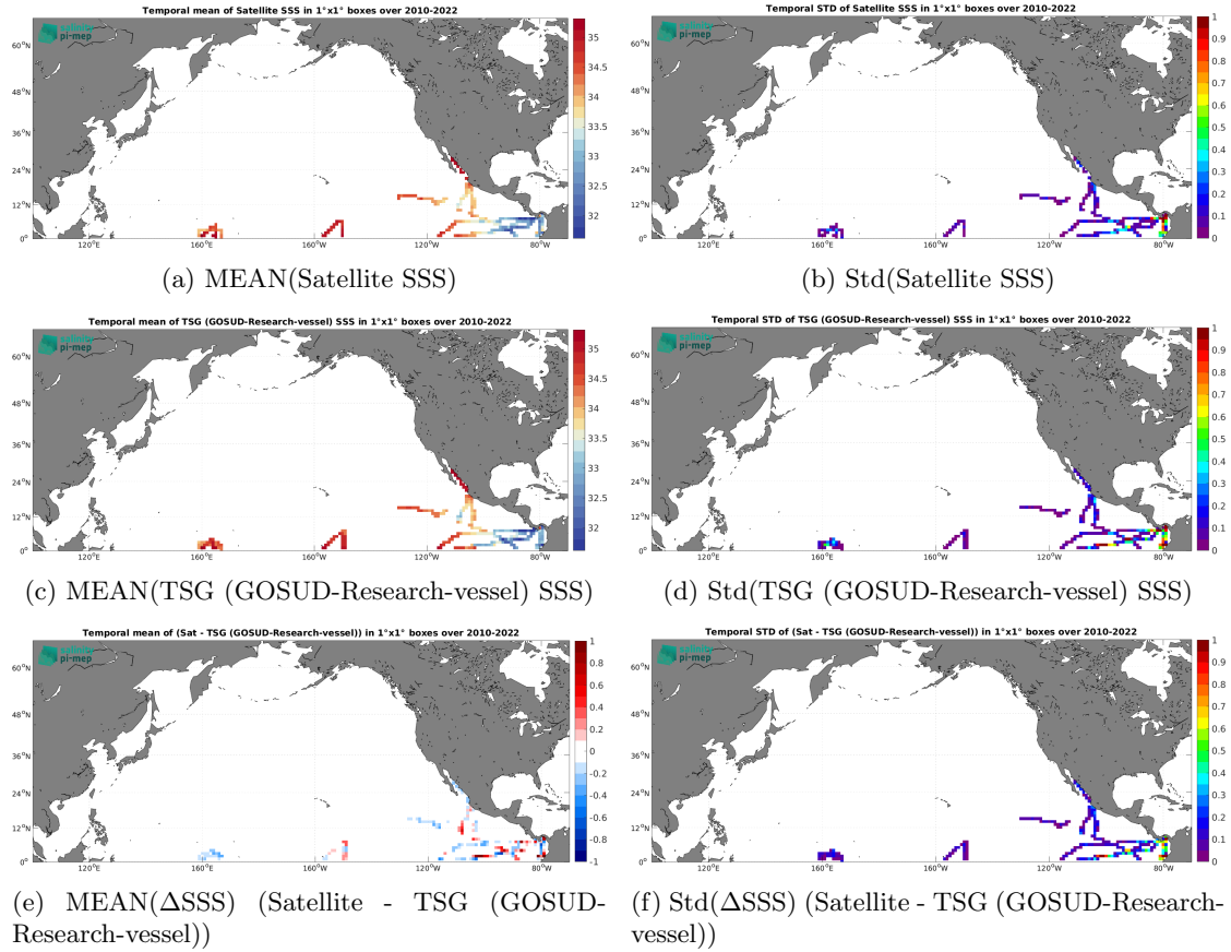
Figure 7: Temporal mean (left) and Std (right) of SSS from SMOS SSS L3 v335 - Monthly - 25 km (CATDS-CPDC) (top), TSG (GOSUD-Research-vessel) (middle), and of \Delta SSS (Satellite - TSG (GOSUD-Research-vessel)). Only match-up pairs are used to generate these maps.
