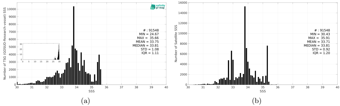
Figure 3: Histograms of SSS from TSG (GOSUD-Research-vessel) (a) and SMOS SSS L3 v335 - Monthly - 25 km (CATDS-CPDC) (b) considering all match-up pairs per bins of 0.1 over the North Pacific Ocean Pi-MEP region and for the full satellite product period.
