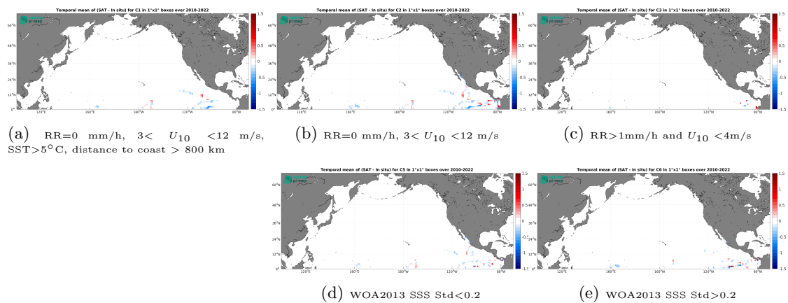
Figure 14: Temporal mean gridded over spatial boxes of size 1^\circ \times 1^\circ of \Delta\text{SSS} (SMOS SSS L3 v335 - Monthly - 25 km (CATDS-CPDC) - TSG (GOSUD-Research-vessel)) for 5 different subdatasets corresponding to:RR=0 mm/h, 3 < U_{10} < 12 m/s, SST>5°C, distance to coast > 800 km (a), RR=0 mm/h, 3 < U_{10} < 12 m/s (b), RR>1mm/h and U_{10} < 4 m/s (c), WOA2013 SSS Std<0.2 (d), WOA2013 SSS Std>0.2 (e).
