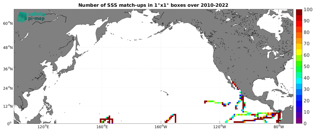
Figure 5: Number of SSS match-ups between TSG (GOSUD-Research-vessel) SSS and the SMOS SSS L3 v335 - Monthly - 25 km (CATDS-CPDC) SSS product for the North Pacific Ocean Pi-MEP region over 1^\circ \times 1^\circ boxes and for the full satellite product period.
