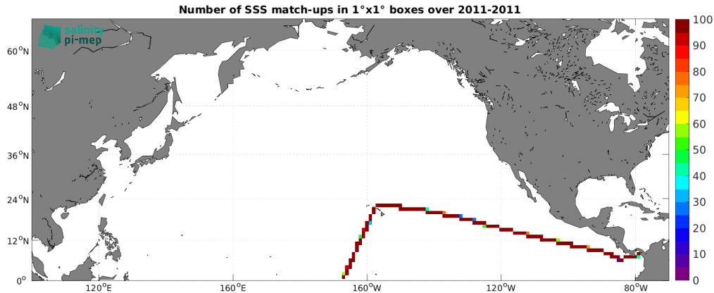
Figure 5: Number of SSS match-ups between TSG (CSIC-UTM) SSS and the SMOS SSS L3 v335 - Monthly - 25 km (CATDS-CPDC) SSS product for the North Pacific Ocean Pi-MEP region over 1^\circ \times 1^\circ boxes and for the full satellite product period.
