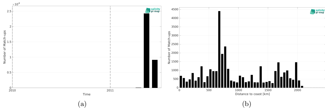
Figure 2: Number of match-ups between TSG (CSIC-UTM) and SMOS SSS L3 v335 - Monthly - 25 km (CATDS-CPDC) SSS as a function of time (a) and as function of the distance to coast (b) over the North Pacific Ocean Pi-MEP region and for the full satellite product period.
