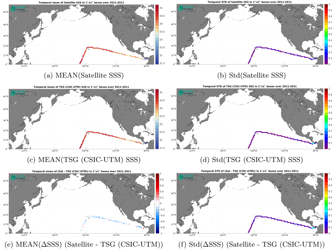
Figure 7: Temporal mean (left) and Std (right) of SSS from SMOS SSS L3 v335 - Monthly - 25 km (CATDS-CPDC) (top), TSG (CSIC-UTM) (middle), and of \Delta\text{SSS} (Satellite - TSG (CSIC-UTM)). Only match-up pairs are used to generate these maps.
