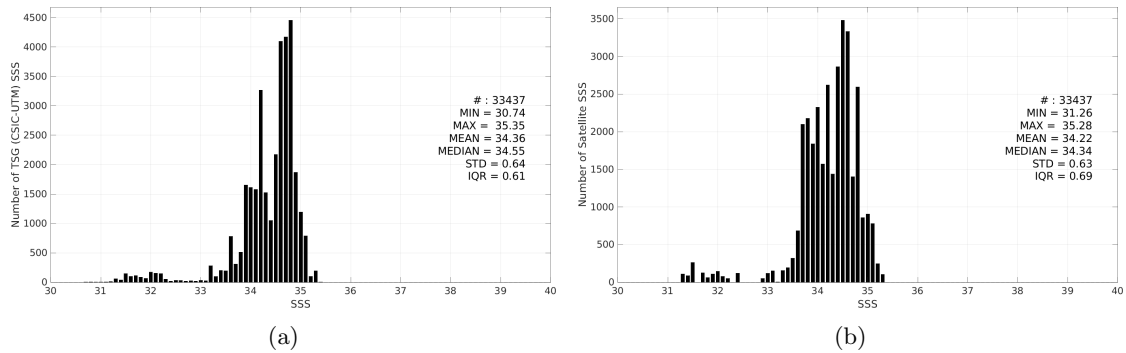
Figure 3: Histograms of SSS from TSG (CSIC-UTM) (a) and SMOS SSS L3 v335 - Monthly - 25 km (CATDS-CPDC) (b) considering all match-up pairs per bins of 0.1 over the North Pacific Ocean Pi-MEP region and for the full satellite product period.
