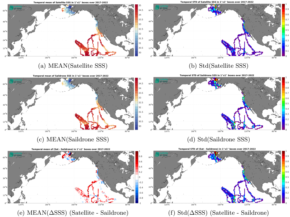
Figure 7: Temporal mean (left) and Std (right) of SSS from SMOS SSS L3 v335 - Monthly - 25 km (CATDS-CPDC) (top), Saildrone (middle), and of \Delta SSS (Satellite - Saildrone). Only match-up pairs are used to generate these maps.
