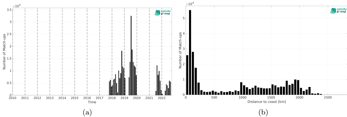
Figure 2: Number of match-ups between Saildrone and SMOS SSS L3 v335 - Monthly - 25 km (CATDS-CPDC) SSS as a function of time (a) and as function of the distance to coast (b) over the North Pacific Ocean Pi-MEP region and for the full satellite product period.
