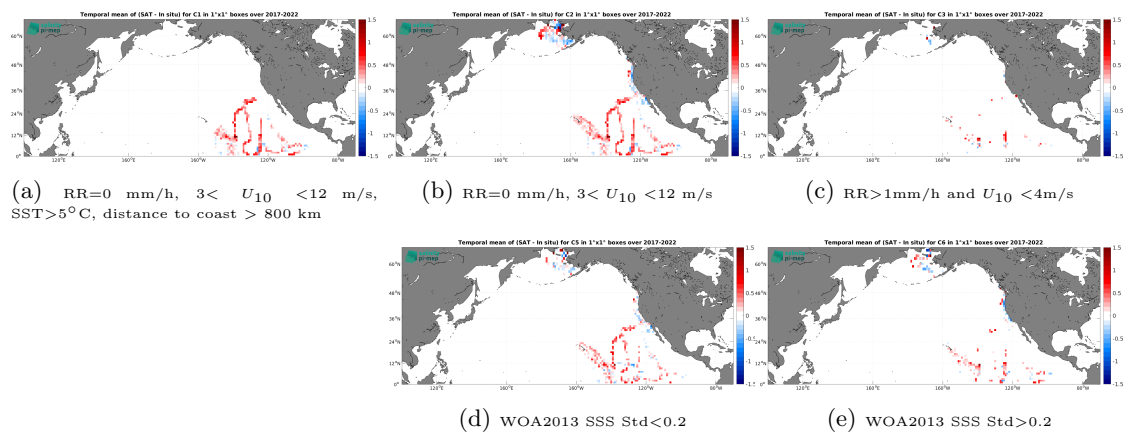
Figure 14: Temporal mean gridded over spatial boxes of size 1^\circ \times 1^\circ of \Delta SSS (SMOS SSS L3 v335 - Monthly - 25 km (CATDS-CPDC) - Saldrone) for 5 different subdatasets corresponding to: RR=0 mm/h, 3 < U_{10} < 12 m/s, SST > 5°C, distance to coast > 800 km (a), RR=0 mm/h, 3 < U_{10} < 12 m/s (b), RR > 1 mm/h and U_{10} < 4 m/s (c), WOA2013 SSS Std < 0.2 (d), WOA2013 SSS Std > 0.2 (e).
