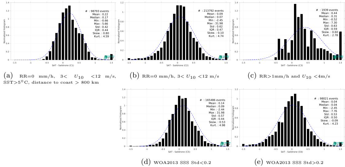
Figure 15: Normalized histogram of \Delta SSS (SMOS SSS L3 v335 - Monthly - 25 km (CATDS-CPDC) - Ssaldrone) for 5 different subdatasets corresponding to: RR=0 mm/h, 3 < U_{10} < 12 m/s, SST>5°C, distance to coast > 800 km (a), RR=0 mm/h, 3 < U_{10} < 12 m/s (b), RR>1mm/h and U_{10} < 4 m/s (c), WOA2013 SSS Std<0.2 (d), WOA2013 SSS Std>0.2 (e).
