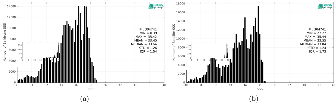
Figure 3: Histograms of SSS from Saildrone (a) and SMOS SSS L3 v335 - Monthly - 25 km (CATDS-CPDC) (b) considering all match-up pairs per bins of 0.1 over the North Pacific Ocean Pi-MEP region and for the full satellite product period.
