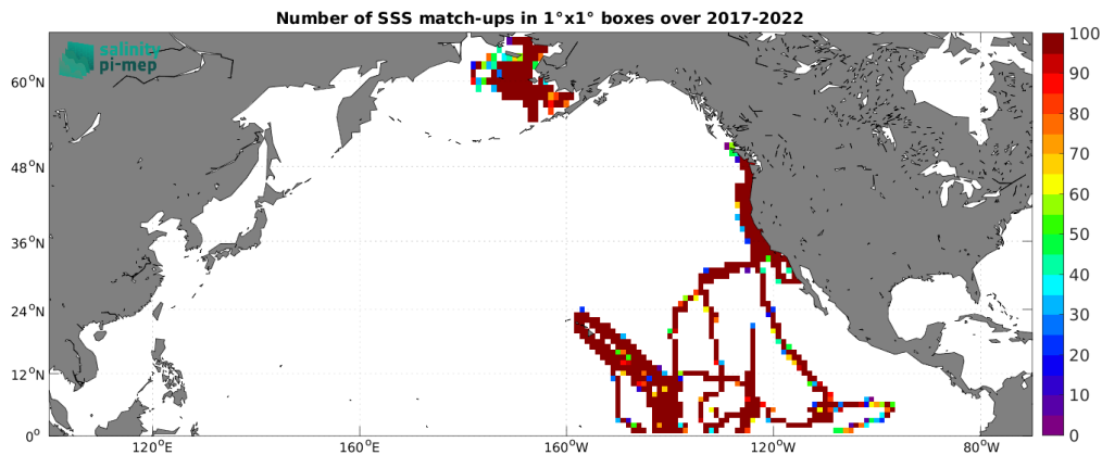
Figure 5: Number of SSS match-ups between Saildrone SSS and the SMOS SSS L3 v335 - Monthly - 25 km (CATDS-CPDC) SSS product for the North Pacific Ocean Pi-MEP region over 1^\circ \times 1^\circ boxes and for the full satellite product period.
