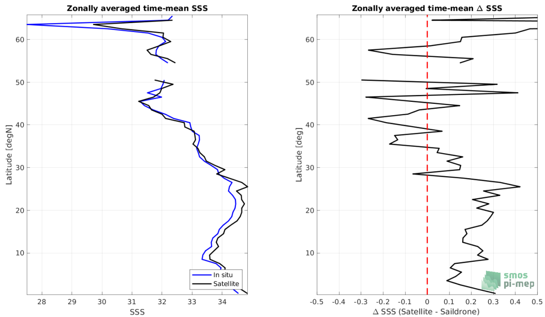
Figure 8: Left panel: Zonal mean SSS from SMOS SSS L3 v335 - Monthly - 25 km (CATDS-CPDC) satellite product (black) and from Sairdron (blue). Right panel: Zonal mean of \Delta SSS (Satellite - Sairdron) for all the collected Pi-MEP match-up pairs estimated over the full satellite product period.
