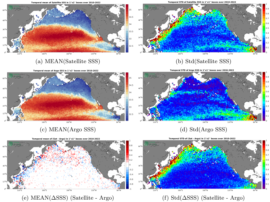
Figure 6: Temporal mean (left) and Std (right) of SSS from SMOS SSS L3 v335 - Monthly - 25 km (CATDS-CPDC) (top), Argo (middle), and of \Delta SSS (Satellite - Argo). Only match-up pairs are used to generate these maps.
