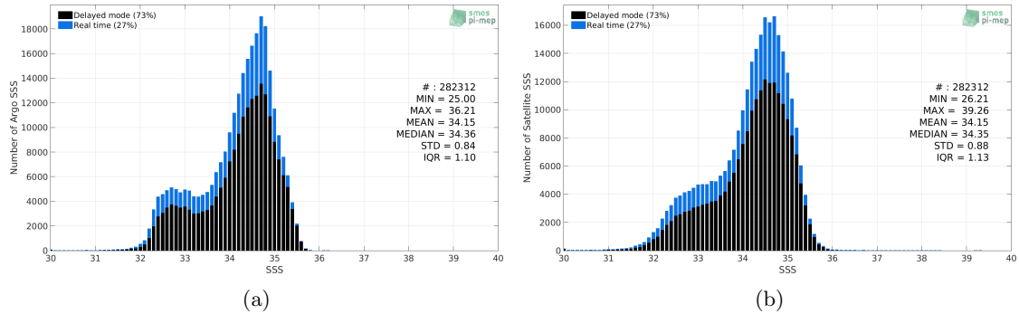
Figure 2: Histograms of SSS from Argo (a) and SMOS SSS L3 v335 - Monthly - 25 km (CATDS-CPDC) (b) considering all match-up pairs per bins of 0.1 over the North Pacific Ocean Pi-MEP region and for the full satellite product period.
