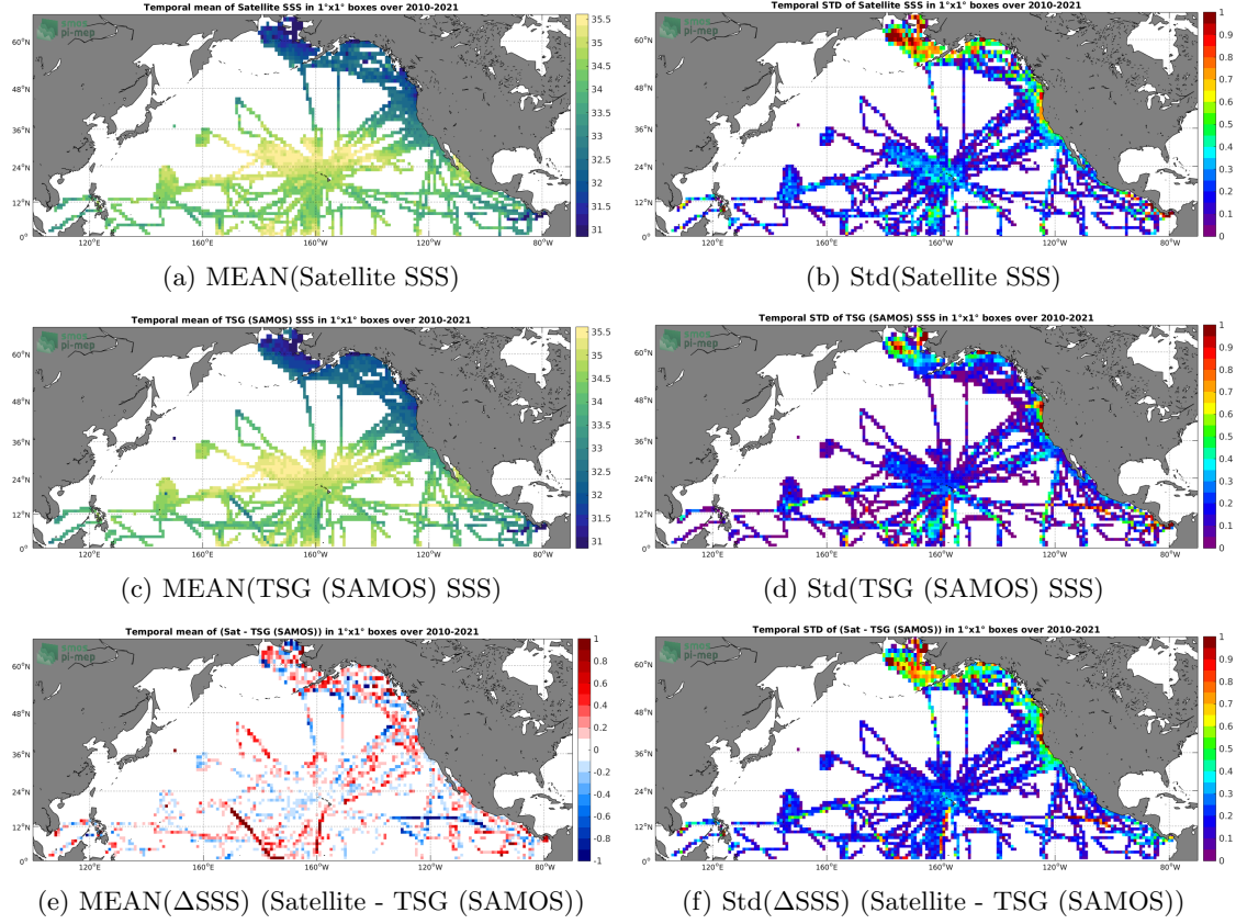
Figure 6: Temporal mean (left) and Std (right) of SSS from SMOS SSS L3 v335 - 10 Days - 25 km (CATDS-CPDC) (top), TSG (SAMOS) (middle), and of \Delta SSS (Satellite - TSG (SAMOS)). Only match-up pairs are used to generate these maps.
