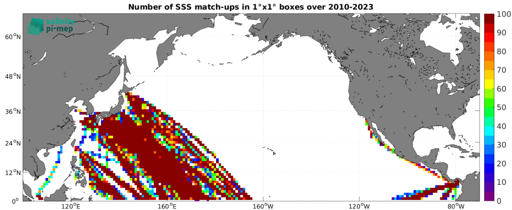
Figure 5: Number of SSS match-ups between TSG (LEGOS-DM) SSS and the SMOS SSS L3 v335 - 10 Days - 25 km (CATDS-CPDC) SSS product for the North Pacific Ocean Pi-MEP region over 1^\circ \times 1^\circ boxes and for the full satellite product period.
