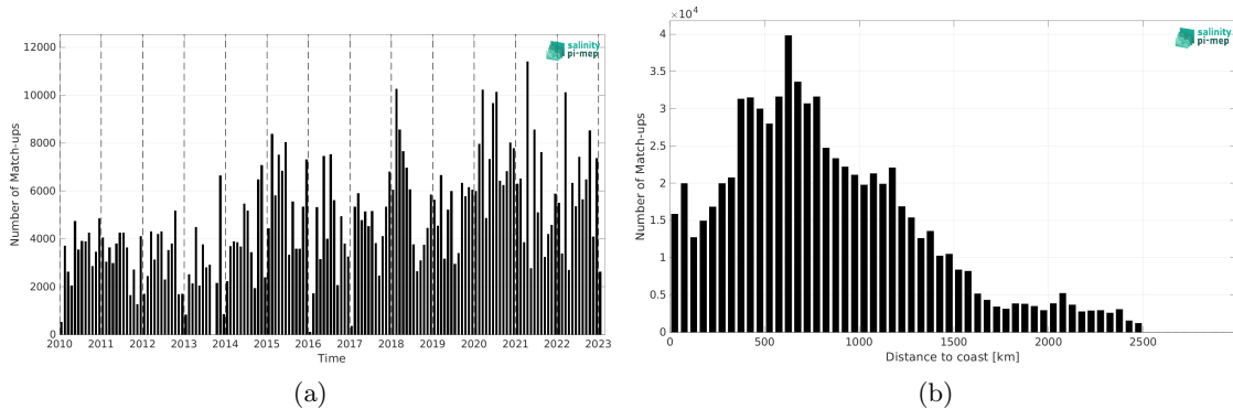
Figure 2: Number of match-ups between TSG (LEGOS-DM) and SMOS SSS L3 v335 - 10 Days - 25 km (CATDS-CPDC) SSS as a function of time (a) and as function of the distance to coast (b) over the North Pacific Ocean Pi-MEP region and for the full satellite product period.
