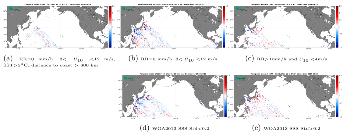
Figure 14: Temporal mean gridded over spatial boxes of size 1^\circ \times 1^\circ of \Delta SSS (SMOS SSS L3 v335 - 10 Days - 25 km (CATDS-CPDC) - TSG (LEGOS-DM)) for 5 different subdatasets corresponding to:RR=0 mm/h, 3 < U_{10} < 12 m/s, SST >5^\circ\text{C} , distance to coast > 800 km (a), RR=0 mm/h, 3 < U_{10} < 12 m/s (b), RR >1 mm/h and U_{10} < 4 m/s (c), WOA2013 SSS Std <0.2 (d), WOA2013 SSS Std >0.2 (e).
