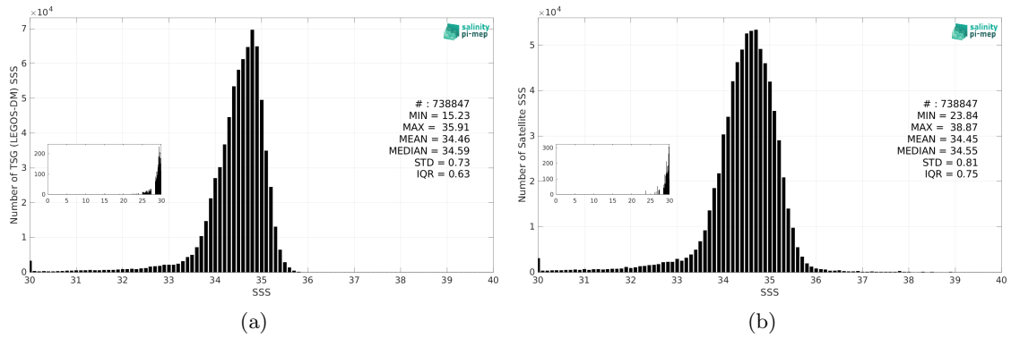
Figure 3: Histograms of SSS from TSG (LEGOS-DM) (a) and SMOS SSS L3 v335 - 10 Days - 25 km (CATDS-CPDC) (b) considering all match-up pairs per bins of 0.1 over the North Pacific Ocean Pi-MEP region and for the full satellite product period.
