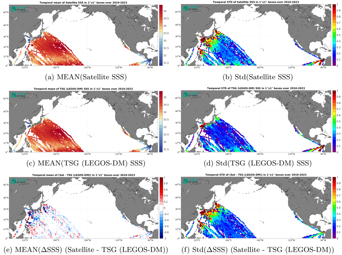
Figure 7: Temporal mean (left) and Std (right) of SSS from SMOS SSS L3 v335 - 10 Days - 25 km (CATDS-CPDC) (top), TSG (LEGOS-DM) (middle), and of \Delta\text{SSS} (Satellite - TSG (LEGOS-DM)). Only match-up pairs are used to generate these maps.
