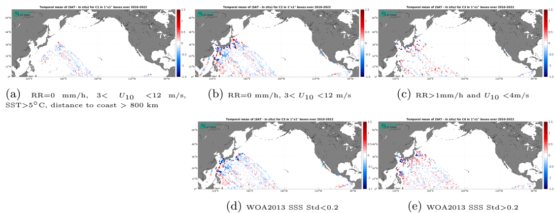
Figure 14: Temporal mean gridded over spatial boxes of size 1^\circ \times 1^\circ of \Delta\text{SSS} (SMOS SSS L3 v335 - 10 Days - 25 km (CATDS-CPDC) - TSG (LEGOS-DM)) for 5 different subdatasets corresponding to: RR=0 mm/h, 3 < U_{10} < 12 m/s, SST > 5°C, distance to coast > 800 km (a), RR=0 mm/h, 3 < U_{10} < 12 m/s (b), RR > 1 mm/h and U_{10} < 4 m/s (c), WOA2013 SSS Std < 0.2 (d), WOA2013 SSS Std > 0.2 (e).
