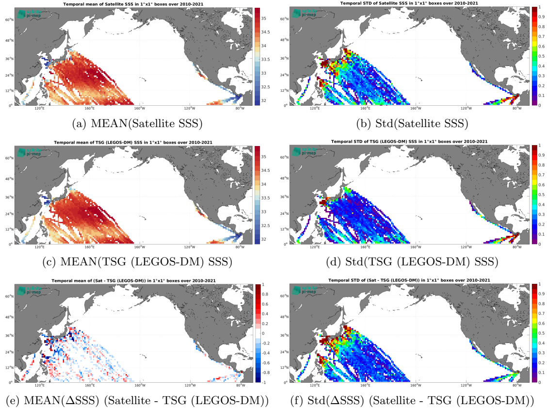
Figure 6: Temporal mean (left) and Std (right) of SSS from SMOS SSS L3 v335 - 10 Days - 25 km (CATDS-CPDC) (top), TSG (LEGOS-DM) (middle), and of \Delta\text{SSS} (Satellite - TSG (LEGOS-DM)). Only match-up pairs are used to generate these maps.
