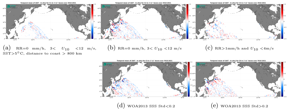
Figure 12: Temporal mean gridded over spatial boxes of size 1^\circ \times 1^\circ of \Delta\text{SSS} (SMOS SSS L3 v335 - 10 Days - 25 km (CATDS-CPDC) - TSG (LEGOS-DM)) for 5 different subdatasets corresponding to:RR=0 mm/h, 3 < U_{10} < 12 m/s, SST >5^\circ\text{C} , distance to coast > 800 km (a), RR=0 mm/h, 3 < U_{10} < 12 m/s (b), RR >1 mm/h and U_{10} < 4 m/s (c), WOA2013 SSS Std <0.2 (d), WOA2013 SSS Std >0.2 (e).
