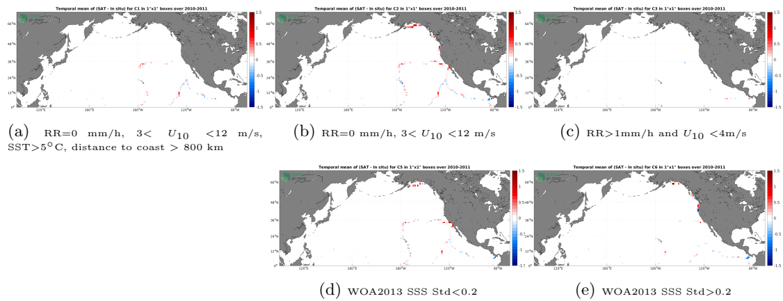
Figure 12: Temporal mean gridded over spatial boxes of size 1^\circ \times 1^\circ of \Delta\text{SSS} (SMOS SSS L3 v335 - 10 Days - 25 km (CATDS-CPDC) - TSG (GOSUD-Sailing-ship)) for 5 different subdatasets corresponding to: RR=0 mm/h, 3 < U_{10} < 12 m/s, SST > 5°C, distance to coast > 800 km (a), RR=0 mm/h, 3 < U_{10} < 12 m/s (b), RR > 1 mm/h and U_{10} < 4 m/s (c), WOA2013 SSS Std < 0.2 (d), WOA2013 SSS Std > 0.2 (e).
