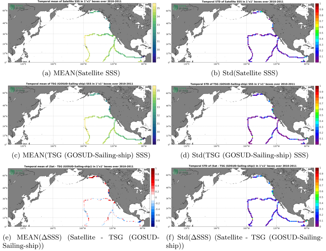
Figure 6: Temporal mean (left) and Std (right) of SSS from SMOS SSS L3 v335 - 10 Days - 25 km (CATDS-CPDC) (top), TSG (GOSUD-Sailing-ship) (middle), and of \Delta SSS (Satellite - TSG (GOSUD-Sailing-ship)). Only match-up pairs are used to generate these maps.
