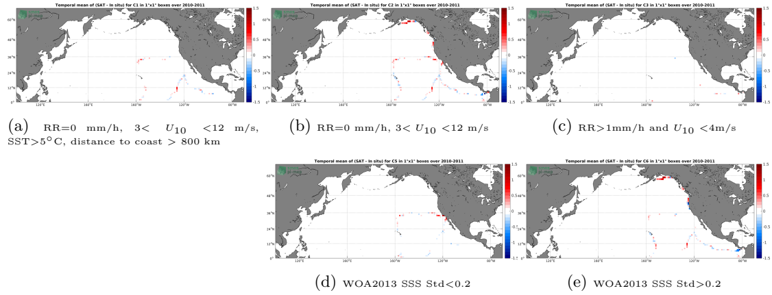
Figure 12: Temporal mean gridded over spatial boxes of size 1^\circ \times 1^\circ of \Delta SSS (SMOS SSS L3 v335 - 10 Days - 25 km (CATDS-CPDC) - TSG (GOSUD-Sailing-ship)) for 5 different subdatasets corresponding to: RR=0 mm/h, 3 < U_{10} < 12 m/s, SST >5^\circ\text{C} , distance to coast > 800 km (a), RR=0 mm/h, 3 < U_{10} < 12 m/s (b), RR >1 mm/h and U_{10} < 4 m/s (c), WOA2013 SSS Std <0.2 (d), WOA2013 SSS Std >0.2 (e).
