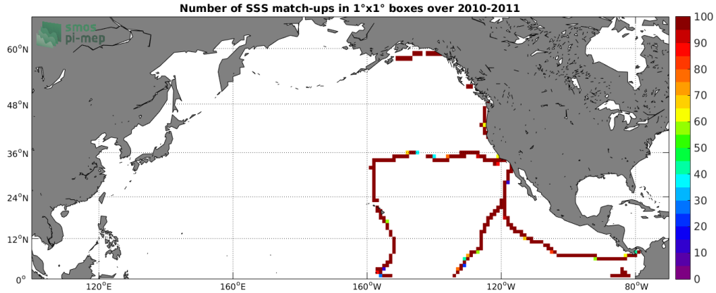
Figure 4: Number of SSS match-ups between TSG (GOSUD-Sailing-ship) SSS and the SMOS SSS L3 v335 - 10 Days - 25 km (CATDS-CPDC) SSS product for the North Pacific Ocean Pi-MEP region over 1^\circ \times 1^\circ boxes and for the full satellite product period.
