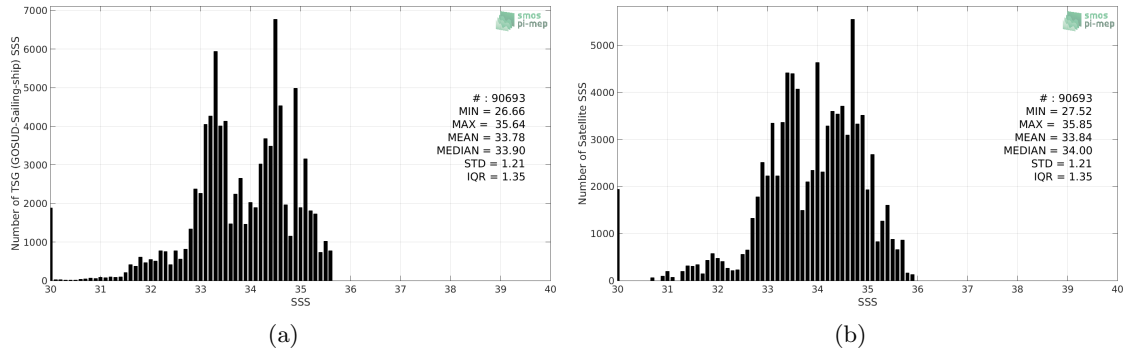
Figure 2: Histograms of SSS from TSG (GOSUD-Sailing-ship) (a) and SMOS SSS L3 v335 - 10 Days - 25 km (CATDS-CPDC) (b) considering all match-up pairs per bins of 0.1 over the North Pacific Ocean Pi-MEP region and for the full satellite product period.
