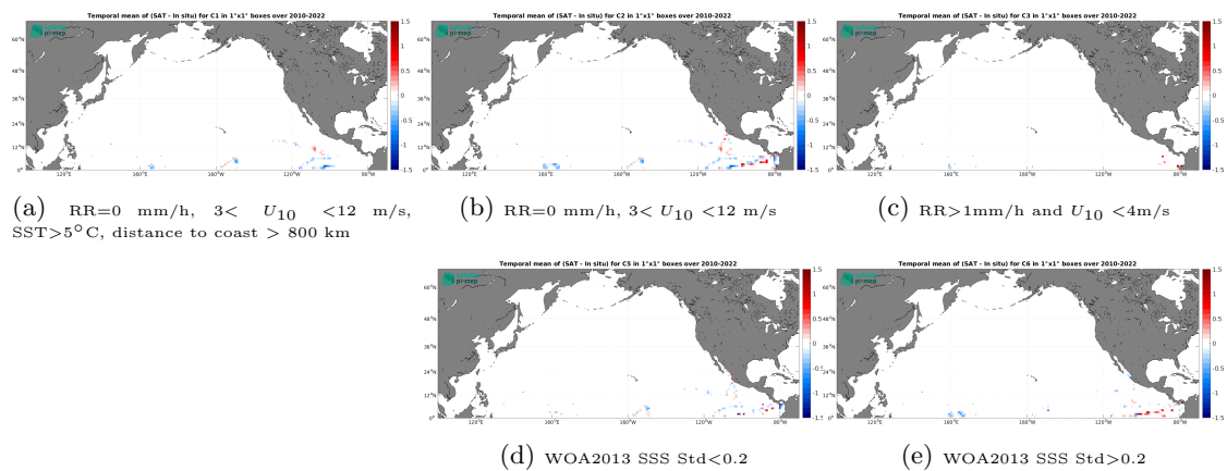
Figure 14: Temporal mean gridded over spatial boxes of size 1^\circ \times 1^\circ of \Delta\text{SSS} (SMOS SSS L3 v335 - 10 Days - 25 km (CATDS-CPDC) - TSG (GOSUD-Research-vessel)) for 5 different subdatasets corresponding to: RR=0 mm/h, 3 < U_{10} < 12 m/s, SST > 5°C, distance to coast > 800 km (a), RR=0 mm/h, 3 < U_{10} < 12 m/s (b), RR > 1 mm/h and U_{10} < 4 m/s (c), WOA2013 SSS Std < 0.2 (d), WOA2013 SSS Std > 0.2 (e).
