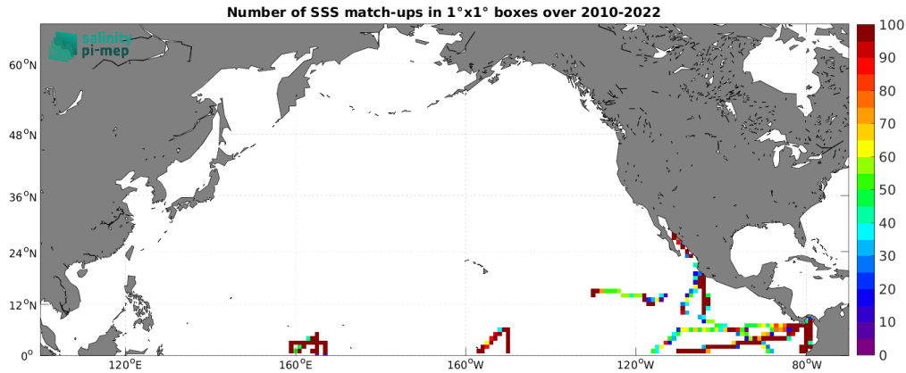
Figure 5: Number of SSS match-ups between TSG (GOSUD-Research-vessel) SSS and the SMOS SSS L3 v335 - 10 Days - 25 km (CATDS-CPDC) SSS product for the North Pacific Ocean Pi-MEP region over 1^\circ \times 1^\circ boxes and for the full satellite product period.
