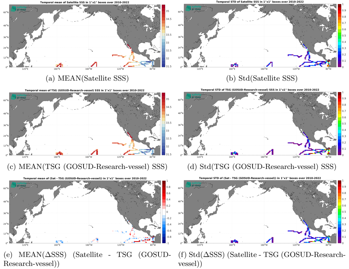
Figure 7: Temporal mean (left) and Std (right) of SSS from SMOS SSS L3 v335 - 10 Days - 25 km (CATDS-CPDC) (top), TSG (GOSUD-Research-vessel) (middle), and of \Delta SSS (Satellite - TSG (GOSUD-Research-vessel)). Only match-up pairs are used to generate these maps.
