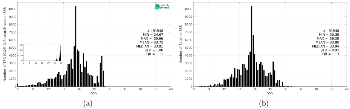
Figure 3: Histograms of SSS from TSG (GOSUD-Research-vessel) (a) and SMOS SSS L3 v335 - 10 Days - 25 km (CATDS-CPDC) (b) considering all match-up pairs per bins of 0.1 over the North Pacific Ocean Pi-MEP region and for the full satellite product period.
