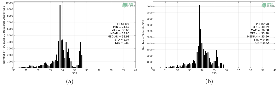
Figure 2: Histograms of SSS from TSG (GOSUD-Research-vessel) (a) and SMOS SSS L3 v335 - 10 Days - 25 km (CATDS-CPDC) (b) considering all match-up pairs per bins of 0.1 over the North Pacific Ocean Pi-MEP region and for the full satellite product period.
