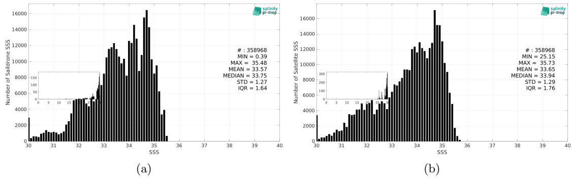
Figure 3: Histograms of SSS from Saildrone (a) and SMOS SSS L3 v335 - 10 Days - 25 km (CATDS-CPDC) (b) considering all match-up pairs per bins of 0.1 over the North Pacific Ocean Pi-MEP region and for the full satellite product period.
