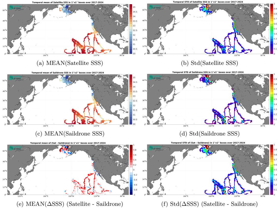
Figure 7: Temporal mean (left) and Std (right) of SSS from SMOS SSS L3 v335 - 10 Days - 25 km (CATDS-CPDC) (top), Saildrone (middle), and of \Delta SSS (Satellite - Saildrone). Only match-up pairs are used to generate these maps.
