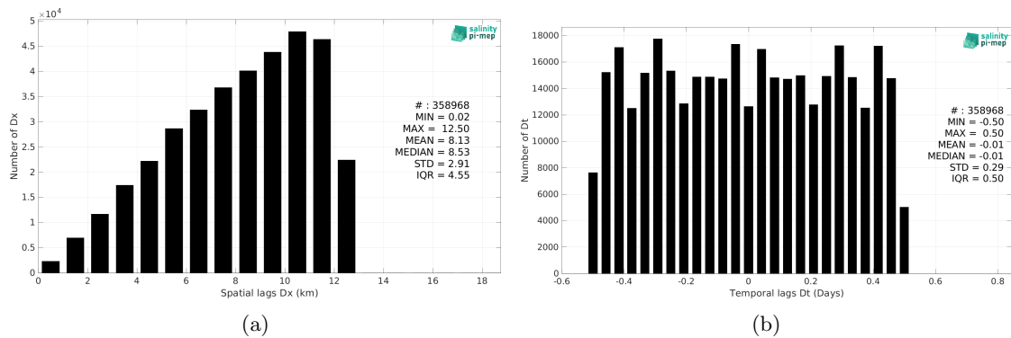
Figure 6: Histograms of the spatial (a) and temporal (b) lags between the location/time of the Sailldrone measurement and the date of the corresponding SMOS SSS L3 v335 - 10 Days - 25 km (CATDS-CPDC) SSS pixel.
