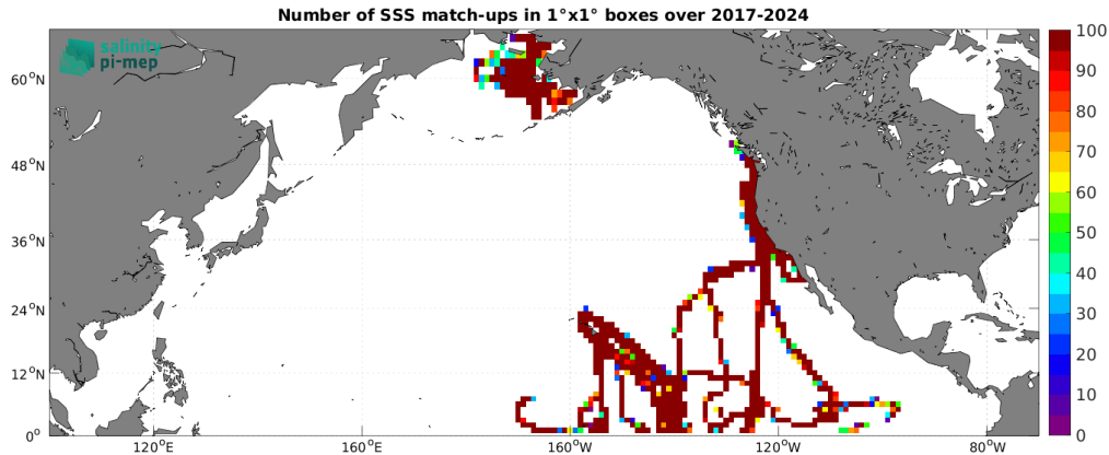
Figure 5: Number of SSS match-ups between Sailldrone SSS and the SMOS SSS L3 v335 - 10 Days - 25 km (CATDS-CPDC) SSS product for the North Pacific Ocean Pi-MEP region over 1^\circ \times 1^\circ boxes and for the full satellite product period.
