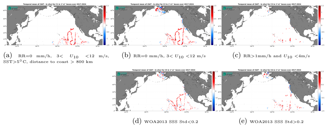
Figure 14: Temporal mean gridded over spatial boxes of size 1^\circ \times 1^\circ of \Delta SSS (SMOS SSS L3 v335 - 10 Days - 25 km (CATDS-CPDC) - Saildrone) for 5 different subdatasets corresponding to:RR=0 mm/h, 3 < U_{10} < 12 m/s, SST>5°C, distance to coast > 800 km (a), RR=0 mm/h, 3 < U_{10} < 12 m/s (b), RR>1mm/h and U_{10} < 4 m/s (c), WOA2013 SSS Std<0.2 (d), WOA2013 SSS Std>0.2 (e).
