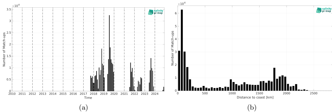
Figure 2: Number of match-ups between Sailability and SMOS SSS L3 v335 - 10 Days - 25 km (CATDS-CPDC) SSS as a function of time (a) and as function of the distance to coast (b) over the North Pacific Ocean Pi-MEP region and for the full satellite product period.
