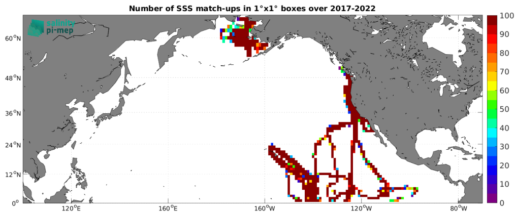
Figure 5: Number of SSS match-ups between Saildrone SSS and the SMOS SSS L3 v335 - 10 Days - 25 km (CATDS-CPDC) SSS product for the North Pacific Ocean Pi-MEP region over 1^\circ \times 1^\circ boxes and for the full satellite product period.
