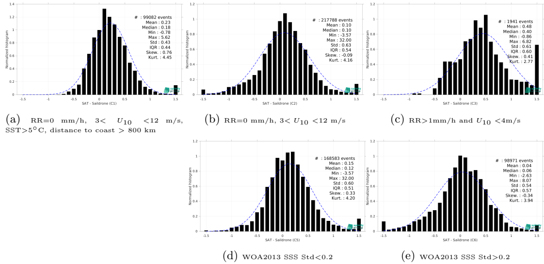
Figure 15: Normalized histogram of \Delta SSS (SMOS SSS L3 v335 - 10 Days - 25 km (CATDS-CPDC) - Saildrone) for 5 different subdatasets corresponding to: RR=0 mm/h, 3 < U_{10} < 12 m/s, SST>5°C, distance to coast > 800 km (a), RR=0 mm/h, 3 < U_{10} < 12 m/s (b), RR>1mm/h and U_{10} < 4 m/s (c), WOA2013 SSS Std<0.2 (d), WOA2013 SSS Std>0.2 (e).
