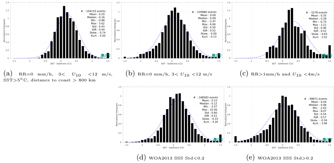
Figure 13: Normalized histogram of \Delta\text{SSS} (SMOS SSS L3 v335 - 10 Days - 25 km (CATDS-CPDC) - Saildrone) for 5 different subdatasets corresponding to: RR=0 mm/h, 3 < U_{10} < 12 m/s, SST>5°C, distance to coast > 800 km (a), RR=0 mm/h, 3 < U_{10} < 12 m/s (b), RR>1mm/h and U_{10} < 4 m/s (c), WOA2013 SSS Std<0.2 (d), WOA2013 SSS Std>0.2 (e).
