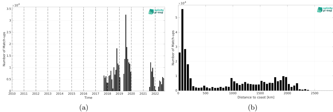
Figure 1: Number of match-ups between Saildrone and SMOS SSS L3 v335 - 10 Days - 25 km (CATDS-CPDC) SSS as a function of time (a) and as function of the distance to coast (b) over the North Pacific Ocean Pi-MEP region and for the full satellite product period.
