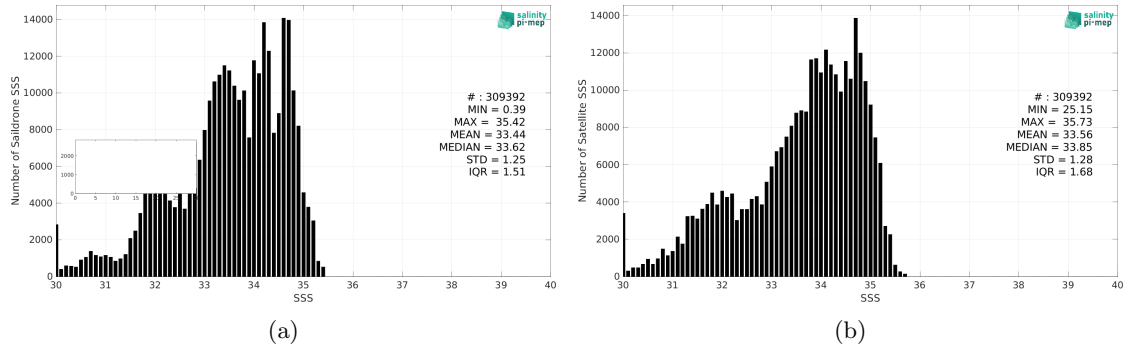
Figure 2: Histograms of SSS from Saildrone (a) and SMOS SSS L3 v335 - 10 Days - 25 km (CATDS-CPDC) (b) considering all match-up pairs per bins of 0.1 over the North Pacific Ocean Pi-MEP region and for the full satellite product period.
