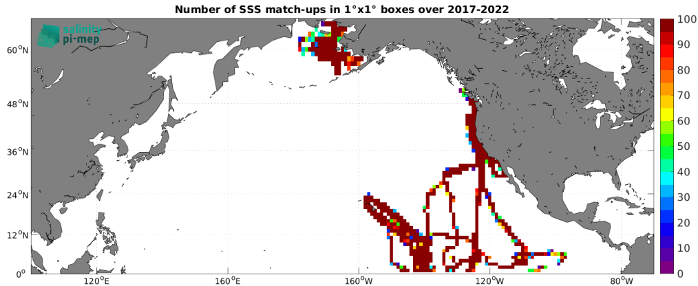
Figure 4: Number of SSS match-ups between Saildrone SSS and the SMOS SSS L3 v335 - 10 Days - 25 km (CATDS-CPDC) SSS product for the North Pacific Ocean Pi-MEP region over 1^\circ \times 1^\circ boxes and for the full satellite product period.
