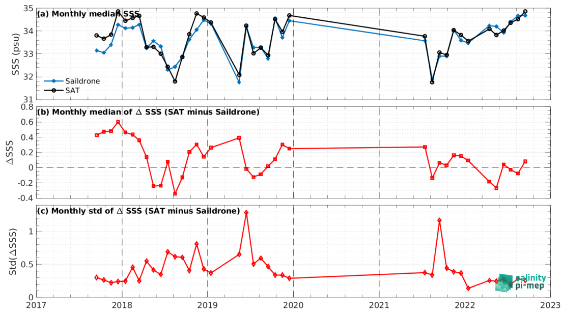
Figure 7: Time series of the monthly median SSS (top), median of \Delta SSS (Satellite - Sairdron) and Std of \Delta SSS (Satellite - Sairdron) over the North Pacific Ocean Pi-MEP region considering all match-ups collected by the Pi-MEP.
