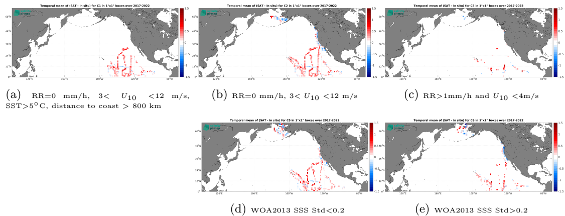
Figure 12: Temporal mean gridded over spatial boxes of size 1^\circ \times 1^\circ of \Delta SSS (SMOS SSS L3 v335 - 10 Days - 25 km (CATDS-CPDC) - Saildrone) for 5 different subdatasets corresponding to:RR=0 mm/h, 3 < U_{10} < 12 m/s, SST >5^\circ C, distance to coast > 800 km (a), RR=0 mm/h, 3 < U_{10} < 12 m/s (b), RR >1 mm/h and U_{10} < 4 m/s (c), WOA2013 SSS Std <0.2 (d), WOA2013 SSS Std >0.2 (e).
