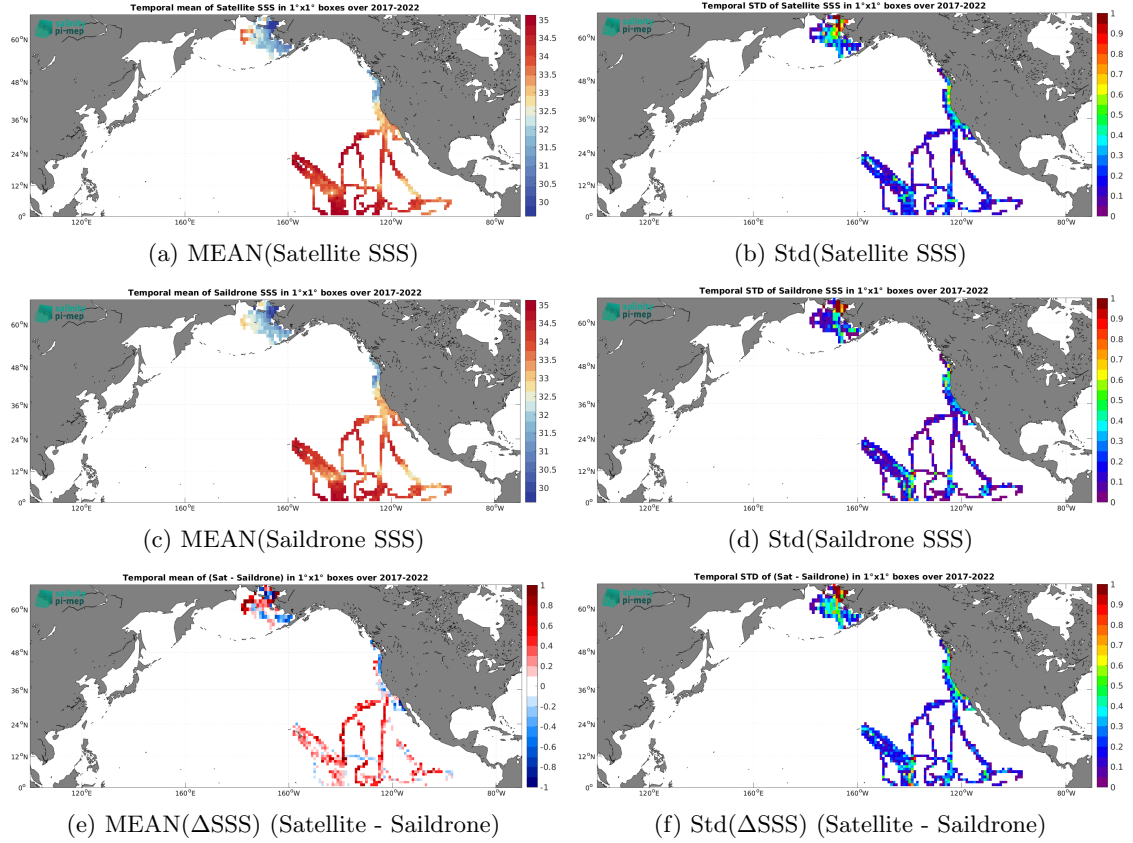
Figure 6: Temporal mean (left) and Std (right) of SSS from SMOS SSS L3 v335 - 10 Days - 25 km (CATDS-CPDC) (top), Saildrone (middle), and of \Delta SSS (Satellite - Saildrone). Only match-up pairs are used to generate these maps.
