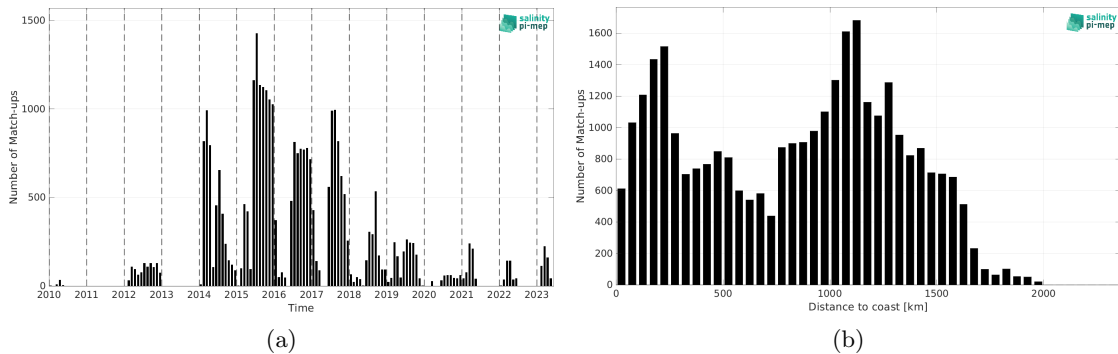
Figure 2: Number of match-ups between Marine mammals and SMOS SSS L3 v335 - 10 Days - 25 km (CATDS-CPDC) SSS as a function of time (a) and as function of the distance to coast (b) over the North Pacific Ocean Pi-MEP region and for the full satellite product period.
