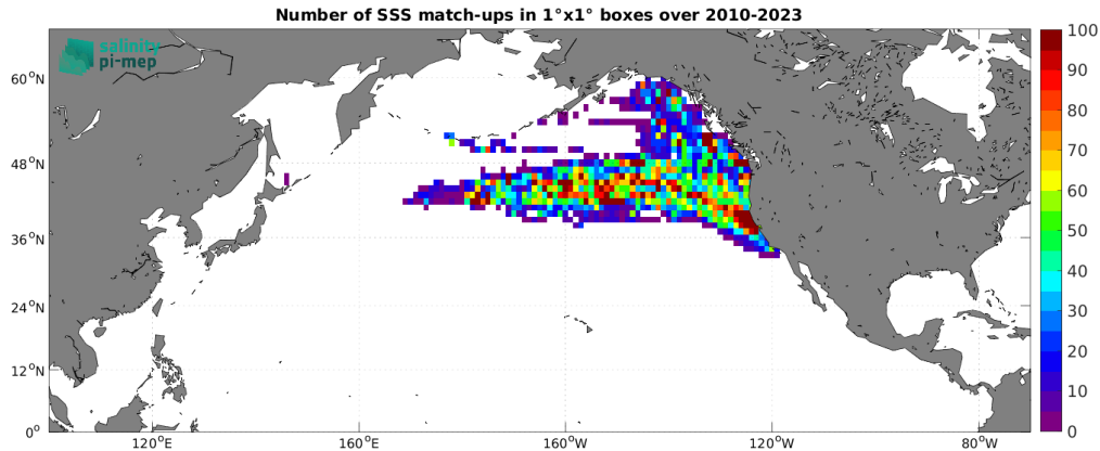
Figure 5: Number of SSS match-ups between Marine mammals SSS and the SMOS SSS L3 v335 - 10 Days - 25 km (CATDS-CPDC) SSS product for the North Pacific Ocean Pi-MEP region over 1^\circ \times 1^\circ boxes and for the full satellite product period.
