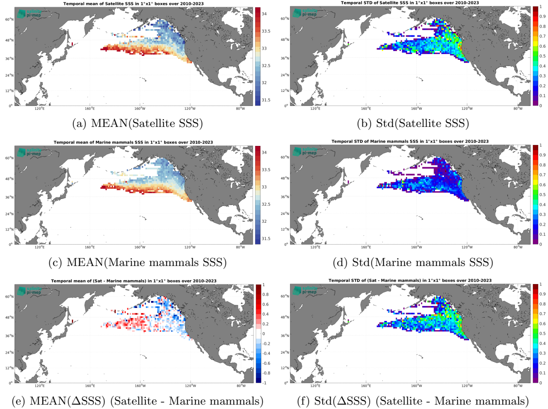
Figure 7: Temporal mean (left) and Std (right) of SSS from SMOS SSS L3 v335 - 10 Days - 25 km (CATDS-CPDC) (top), Marine mammals (middle), and of \Delta SSS (Satellite - Marine mammals). Only match-up pairs are used to generate these maps.
