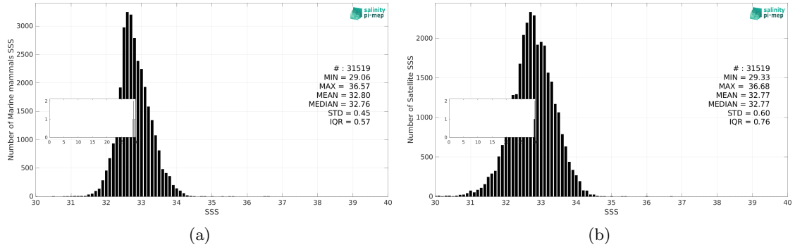
Figure 3: Histograms of SSS from Marine mammals (a) and SMOS SSS L3 v335 - 10 Days - 25 km (CATDS-CPDC) (b) considering all match-up pairs per bins of 0.1 over the North Pacific Ocean Pi-MEP region and for the full satellite product period.
