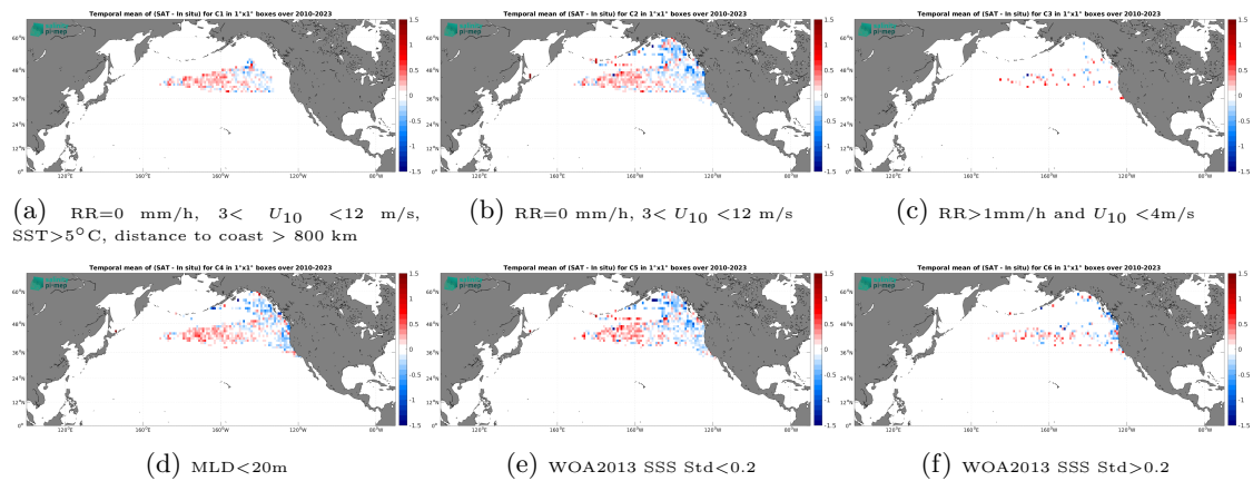
Figure 14: Temporal mean gridded over spatial boxes of size 1^\circ \times 1^\circ of \Delta SSS (SMOS SSS L3 v335 - 10 Days - 25 km (CATDS-CPDC) - Marine mammals) for 6 different subdatasets corresponding to:RR=0 mm/h, 3 < U_{10} < 12 m/s, SST>5°C, distance to coast > 800 km (a), RR=0 mm/h, 3 < U_{10} < 12 m/s (b), RR>1mm/h and U_{10} < 4 m/s (c),MLD<20m (d),WOA2013 SSS Std<0.2 (e),WOA2013 SSS Std>0.2 (f).
