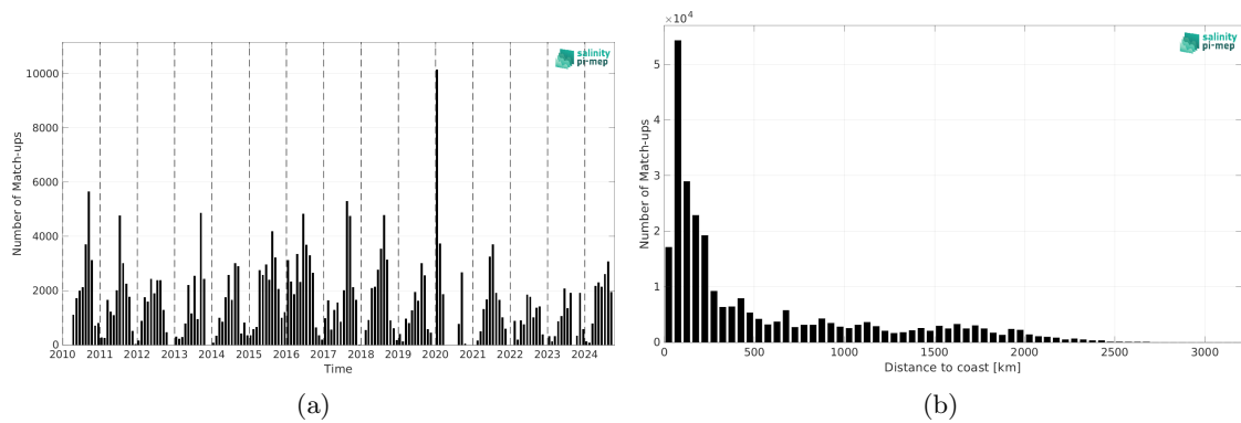
Figure 2: Number of match-ups between TSG (SAMOS) and SMOS SSS L2Q v333 - 0.25 Deg (CATDS-CPDC) SSS as a function of time (a) and as function of the distance to coast (b) over the North Pacific Ocean Pi-MEP region and for the full satellite product period.
