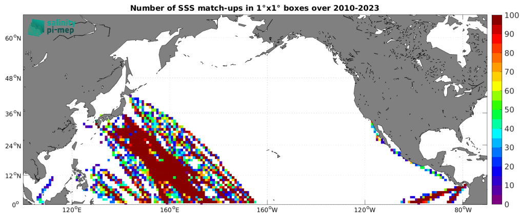
Figure 5: Number of SSS match-ups between TSG (LEGOS-DM) SSS and the SMOS SSS L2Q v333 - 0.25 Deg (CATDS-CPDC) SSS product for the North Pacific Ocean Pi-MEP region over 1^\circ \times 1^\circ boxes and for the full satellite product period.
