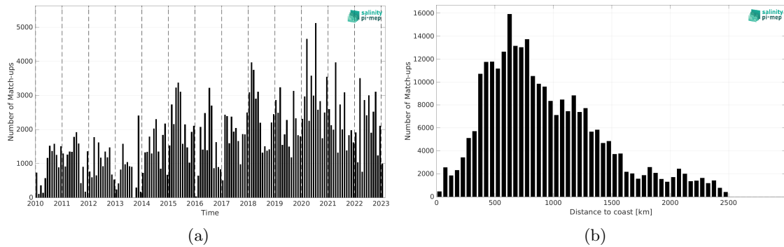
Figure 2: Number of match-ups between TSG (LEGOS-DM) and SMOS SSS L2Q v333 - 0.25 Deg (CATDS-CPDC) SSS as a function of time (a) and as function of the distance to coast (b) over the North Pacific Ocean Pi-MEP region and for the full satellite product period.
