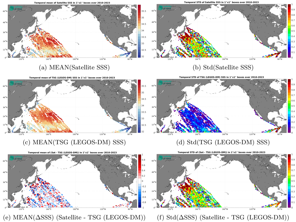
Figure 7: Temporal mean (left) and Std (right) of SSS from SMOS SSS L2Q v333 - 0.25 Deg (CATDS-CPDC) (top), TSG (LEGOS-DM) (middle), and of \Delta SSS (Satellite - TSG (LEGOS-DM)). Only match-up pairs are used to generate these maps.
