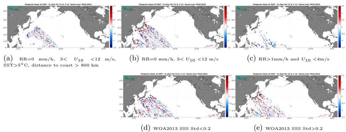
Figure 14: Temporal mean gridded over spatial boxes of size 1^\circ \times 1^\circ of \Delta\text{SSS} (SMOS SSS L2Q v333 - 0.25 Deg (CATDS-CPDC) - TSG (LEGOS-DM)) for 5 different subdatasets corresponding to: RR=0 mm/h, 3 < U_{10} < 12 m/s, SST > 5°C, distance to coast > 800 km (a), RR=0 mm/h, 3 < U_{10} < 12 m/s (b), RR > 1mm/h and U_{10} < 4 m/s (c), WOA2013 SSS Std < 0.2 (d), WOA2013 SSS Std > 0.2 (e).
