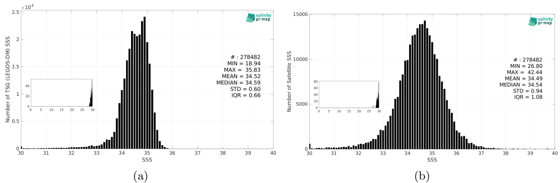
Figure 3: Histograms of SSS from TSG (LEGOS-DM) (a) and SMOS SSS L2Q v333 - 0.25 Deg (CATDS-CPDC) (b) considering all match-up pairs per bins of 0.1 over the North Pacific Ocean Pi-MEP region and for the full satellite product period.
