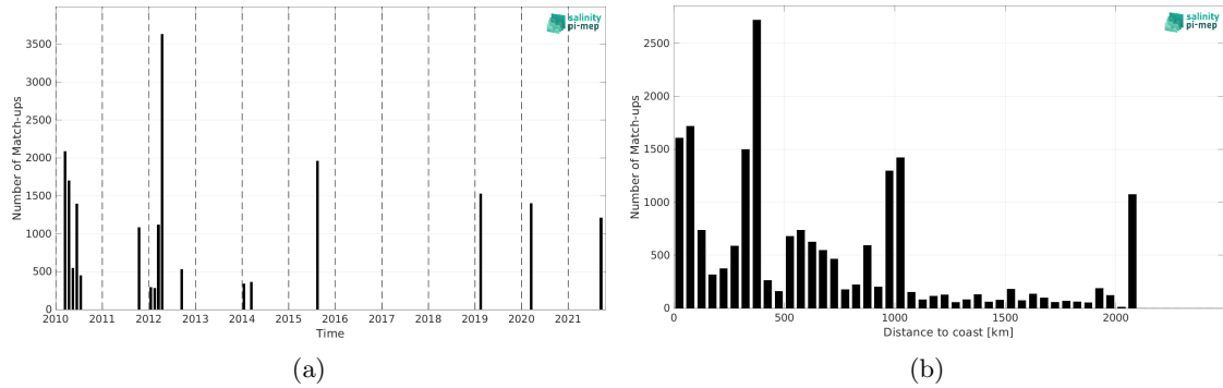
Figure 2: Number of match-ups between TSG (GOSUD-Research-vessel) and SMOS SSS L2Q v333 - 0.25 Deg (CATDS-CPDC) SSS as a function of time (a) and as function of the distance to coast (b) over the North Pacific Ocean Pi-MEP region and for the full satellite product period.
