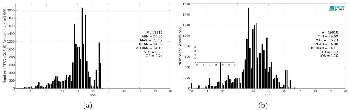
Figure 3: Histograms of SSS from TSG (GOSUD-Research-vessel) (a) and SMOS SSS L2Q v333 - 0.25 Deg (CATDS-CPDC) (b) considering all match-up pairs per bins of 0.1 over the North Pacific Ocean Pi-MEP region and for the full satellite product period.
