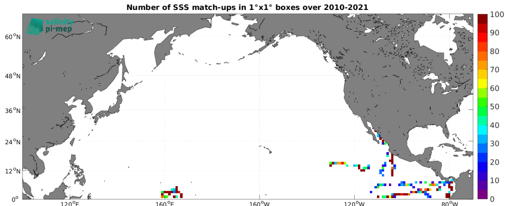
Figure 5: Number of SSS match-ups between TSG (GOSUD-Research-vessel) SSS and the SMOS SSS L2Q v333 - 0.25 Deg (CATDS-CPDC) SSS product for the North Pacific Ocean Pi-MEP region over 1^\circ \times 1^\circ boxes and for the full satellite product period.
