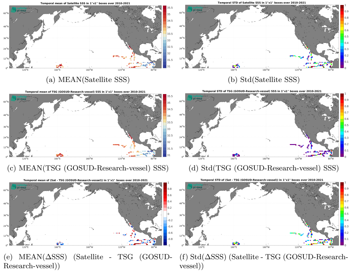
Figure 7: Temporal mean (left) and Std (right) of SSS from SMOS SSS L2Q v333 - 0.25 Deg (CATDS-CPDC) (top), TSG (GOSUD-Research-vessel) (middle), and of \Delta SSS (Satellite - TSG (GOSUD-Research-vessel)). Only match-up pairs are used to generate these maps.
