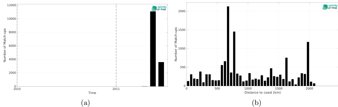
Figure 2: Number of match-ups between TSG (CSIC-UTM) and SMOS SSS L2Q v333 - 0.25 Deg (CATDS-CPDC) SSS as a function of time (a) and as function of the distance to coast (b) over the North Pacific Ocean Pi-MEP region and for the full satellite product period.
