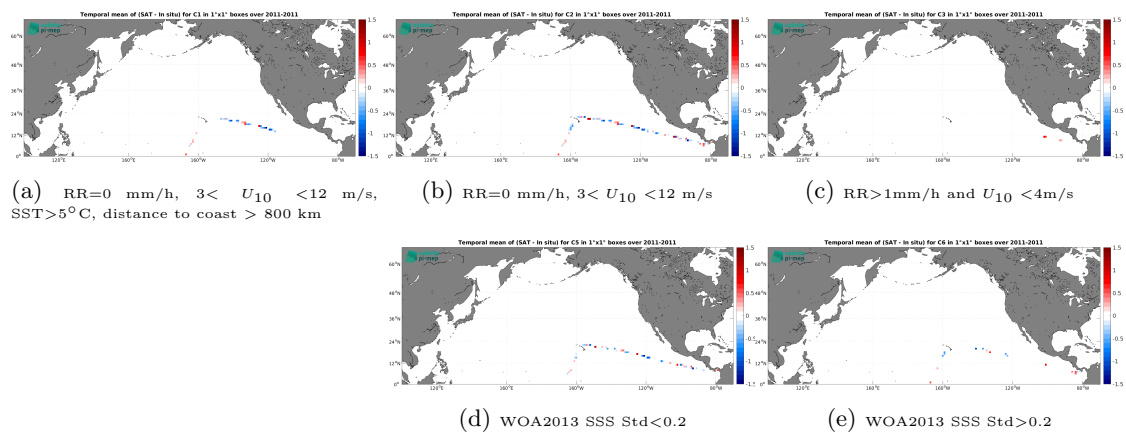
Figure 14: Temporal mean gridded over spatial boxes of size 1^\circ \times 1^\circ of \Delta\text{SSS} (SMOS SSS L2Q v333 - 0.25 Deg (CATDS-CPDC) - TSG (CSIC-UTM)) for 5 different subdatasets corresponding to: RR=0 mm/h, 3 < U_{10} < 12 m/s, SST > 5°C, distance to coast > 800 km (a), RR=0 mm/h, 3 < U_{10} < 12 m/s (b), RR > 1mm/h and U_{10} < 4 m/s (c), WOA2013 SSS Std < 0.2 (d), WOA2013 SSS Std > 0.2 (e).
