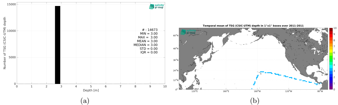
Figure 4: Histograms of the depth of the upper level SSS measurements from TSG (CSIC-UTM) in the Match-up DataBase for the North Pacific Ocean Pi-MEP region (a) and temporal mean spatial distribution of pressure of the in situ SSS data over 1^\circ \times 1^\circ boxes and for the full satellite product period (b).
