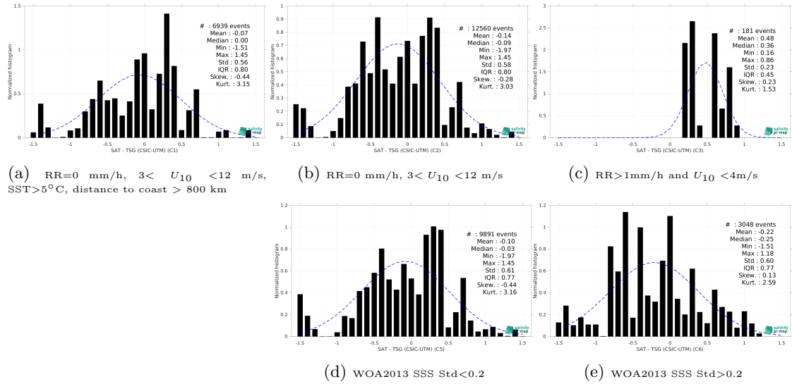
Figure 15: Normalized histogram of \Delta\text{SSS} (SMOS SSS L2Q v333 - 0.25 Deg (CATDS-CPDC) - TSG (CSIC-UTM)) for 5 different subdatasets corresponding to: RR=0 mm/h, 3 < U_{10} < 12 m/s, SST>5°C, distance to coast > 800 km (a), RR=0 mm/h, 3 < U_{10} < 12 m/s (b), RR>1mm/h and U_{10} < 4 m/s (c), WOA2013 SSS Std<0.2 (d), WOA2013 SSS Std>0.2 (e).
