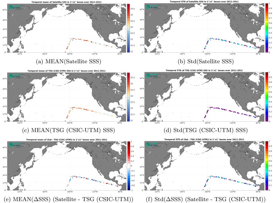
Figure 7: Temporal mean (left) and Std (right) of SSS from SMOS SSS L2Q v333 - 0.25 Deg (CATDS-CPDC) (top), TSG (CSIC-UTM) (middle), and of \Delta\text{SSS} (Satellite - TSG (CSIC-UTM)). Only match-up pairs are used to generate these maps.
