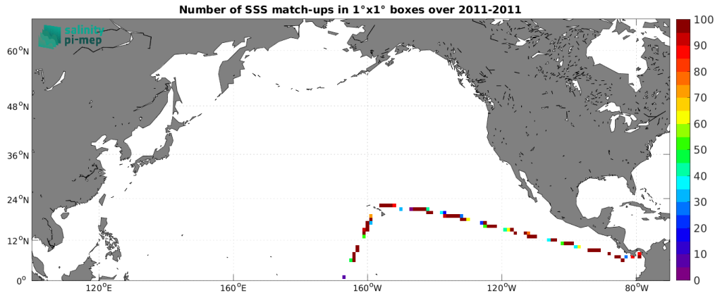
Figure 5: Number of SSS match-ups between TSG (CSIC-UTM) SSS and the SMOS SSS L2Q v333 - 0.25 Deg (CATDS-CPDC) SSS product for the North Pacific Ocean Pi-MEP region over 1^\circ \times 1^\circ boxes and for the full satellite product period.
