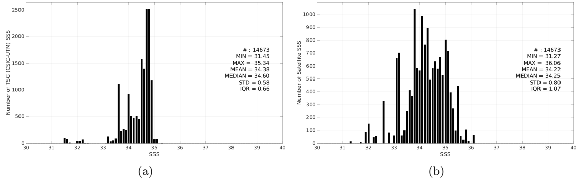
Figure 3: Histograms of SSS from TSG (CSIC-UTM) (a) and SMOS SSS L2Q v333 - 0.25 Deg (CATDS-CPDC) (b) considering all match-up pairs per bins of 0.1 over the North Pacific Ocean Pi-MEP region and for the full satellite product period.
