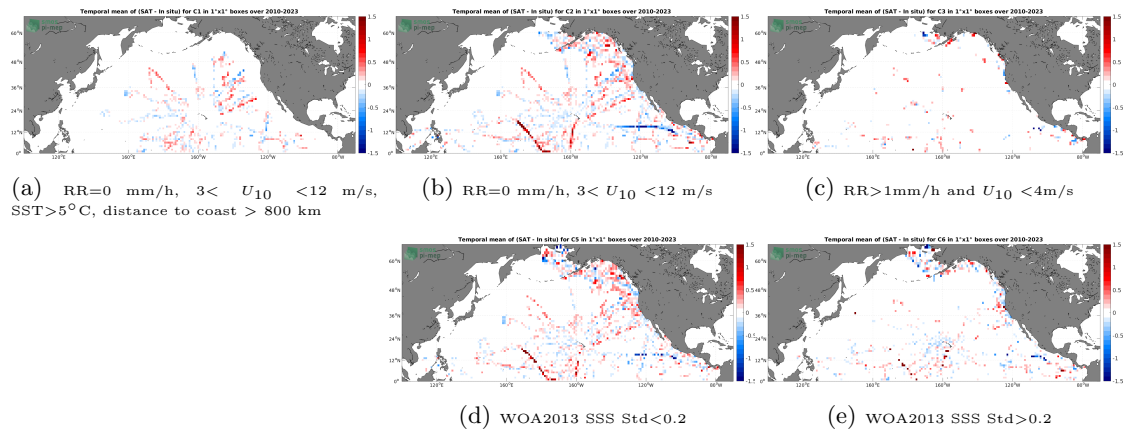
Figure 12: Temporal mean gridded over spatial boxes of size 1^\circ \times 1^\circ of \Delta SSS (SMOS SSS L3 v332 - 9 Days (CATDS-CPDC) - TSG (SAMOS)) for 5 different subdatasets corresponding to:RR=0 mm/h, 3 < U_{10} < 12 m/s, SST > 5^\circ C , distance to coast > 800 km (a), RR=0 mm/h, 3 < U_{10} < 12 m/s (b), RR >1 mm/h and U_{10} < 4 m/s (c), WOA2013 SSS Std <0.2 (d), WOA2013 SSS Std >0.2 (e).
