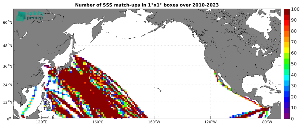
Figure 5: Number of SSS match-ups between TSG (LEGOS-DM) SSS and the SMOS SSS L3 v332 - 9 Days (CATDS-CPDC) SSS product for the North Pacific Ocean Pi-MEP region over 1^\circ \times 1^\circ boxes and for the full satellite product period.
