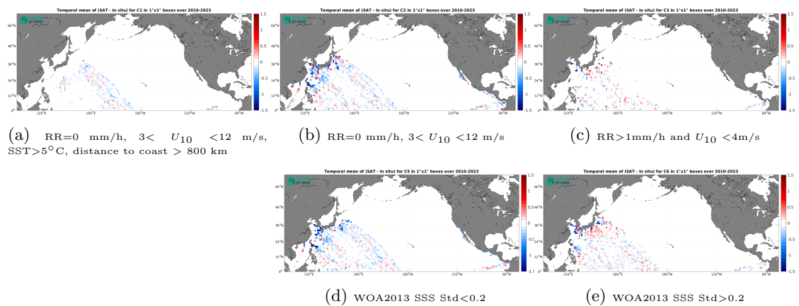
Figure 14: Temporal mean gridded over spatial boxes of size 1^\circ \times 1^\circ of \Delta SSS (SMOS SSS L3 v332 - 9 Days (CATDS-CPDC) - TSG (LEGOS-DM)) for 5 different subdatasets corresponding to:RR=0 mm/h, 3 < U_{10} < 12 m/s, SST > 5°C, distance to coast > 800 km (a), RR=0 mm/h, 3 < U_{10} < 12 m/s (b), RR > 1mm/h and U_{10} < 4 m/s (c), WOA2013 SSS Std < 0.2 (d), WOA2013 SSS Std > 0.2 (e).
