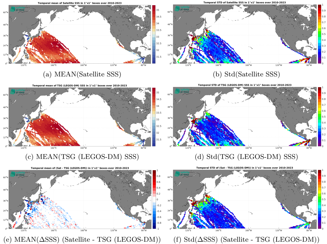
Figure 7: Temporal mean (left) and Std (right) of SSS from SMOS SSS L3 v332 - 9 Days (CATDS-CPDC) (top), TSG (LEGOS-DM) (middle), and of \Delta SSS (Satellite - TSG (LEGOS-DM)). Only match-up pairs are used to generate these maps.
