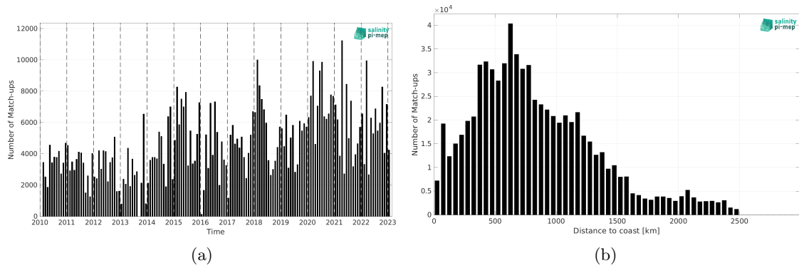
Figure 2: Number of match-ups between TSG (LEGOS-DM) and SMOS SSS L3 v332 - 9 Days (CATDS-CPDC) SSS as a function of time (a) and as function of the distance to coast (b) over the North Pacific Ocean Pi-MEP region and for the full satellite product period.
