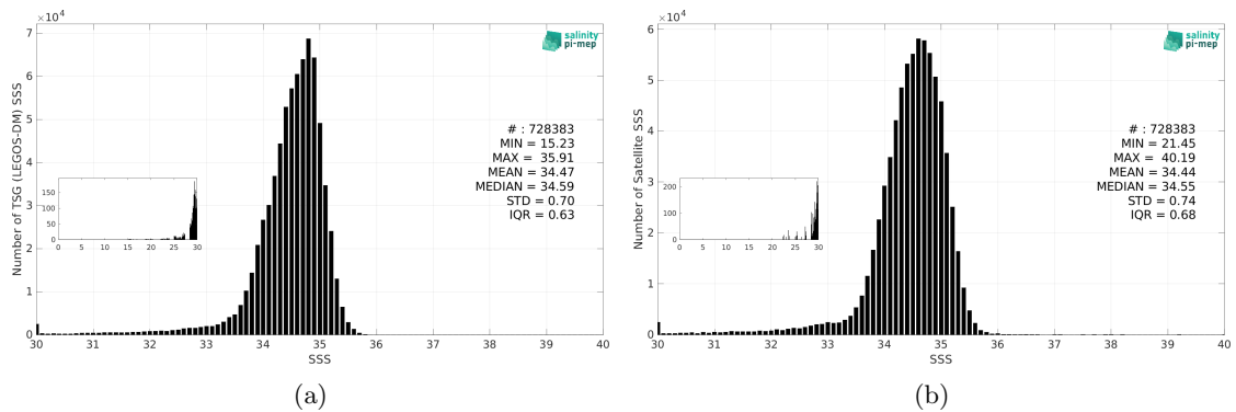
Figure 3: Histograms of SSS from TSG (LEGOS-DM) (a) and SMOS SSS L3 v332 - 9 Days (CATDS-CPDC) (b) considering all match-up pairs per bins of 0.1 over the North Pacific Ocean Pi-MEP region and for the full satellite product period.
