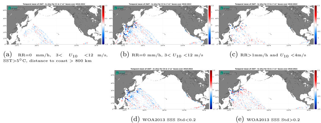
Figure 14: Temporal mean gridded over spatial boxes of size 1^\circ \times 1^\circ of \Delta\text{SSS} (SMOS SSS L3 v332 - 9 Days (CATDS-CPDC) - TSG (LEGOS-DM)) for 5 different subdatasets corresponding to: RR=0 mm/h, 3 < U_{10} < 12 m/s, SST > 5°C, distance to coast > 800 km (a), RR=0 mm/h, 3 < U_{10} < 12 m/s (b), RR > 1mm/h and U_{10} < 4 m/s (c), WOA2013 SSS Std < 0.2 (d), WOA2013 SSS Std > 0.2 (e).
