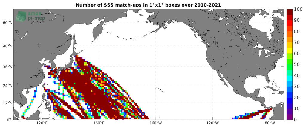
Figure 4: Number of SSS match-ups between TSG (LEGOS-DM) SSS and the SMOS SSS L3 v332 - 9 Days (CATDS-CPDC) SSS product for the North Pacific Ocean Pi-MEP region over 1^\circ \times 1^\circ boxes and for the full satellite product period.
