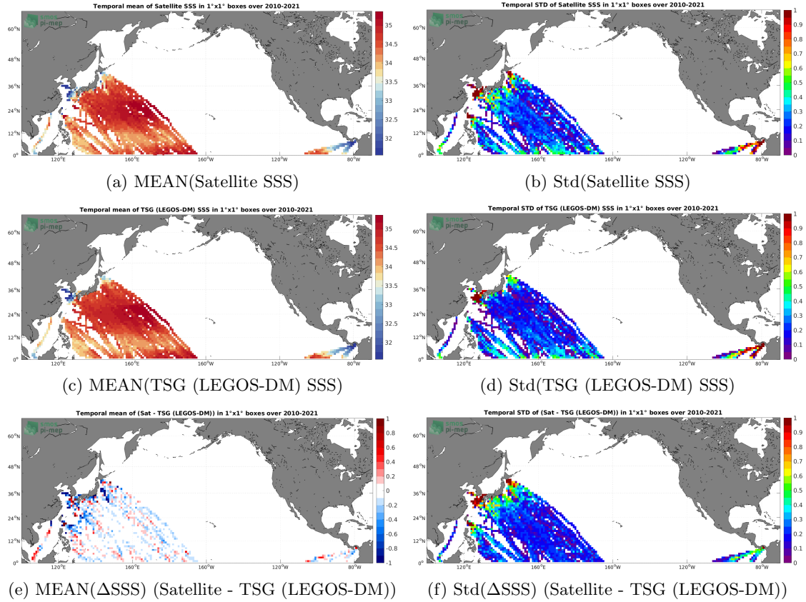
Figure 6: Temporal mean (left) and Std (right) of SSS from SMOS SSS L3 v332 - 9 Days (CATDS-CPDC) (top), TSG (LEGOS-DM) (middle), and of \Delta SSS (Satellite - TSG (LEGOS-DM)). Only match-up pairs are used to generate these maps.
