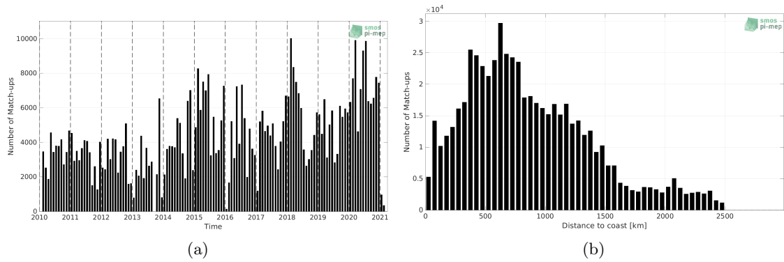
Figure 1: Number of match-ups between TSG (LEGOS-DM) and SMOS SSS L3 v332 - 9 Days (CATDS-CPDC) SSS as a function of time (a) and as function of the distance to coast (b) over the North Pacific Ocean Pi-MEP region and for the full satellite product period.
