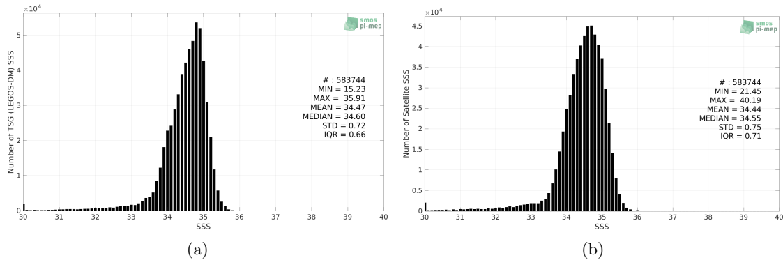
Figure 2: Histograms of SSS from TSG (LEGOS-DM) (a) and SMOS SSS L3 v332 - 9 Days (CATDS-CPDC) (b) considering all match-up pairs per bins of 0.1 over the North Pacific Ocean Pi-MEP region and for the full satellite product period.
