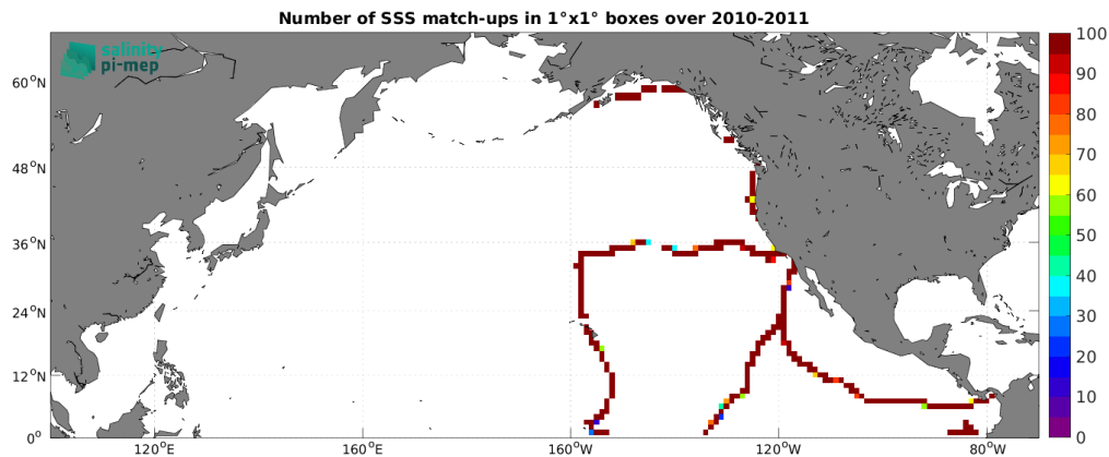
Figure 5: Number of SSS match-ups between TSG (GOSUD-Sailing-ship) SSS and the SMOS SSS L3 v332 - 9 Days (CATDS-CPDC) SSS product for the North Pacific Ocean Pi-MEP region over 1^\circ \times 1^\circ boxes and for the full satellite product period.
