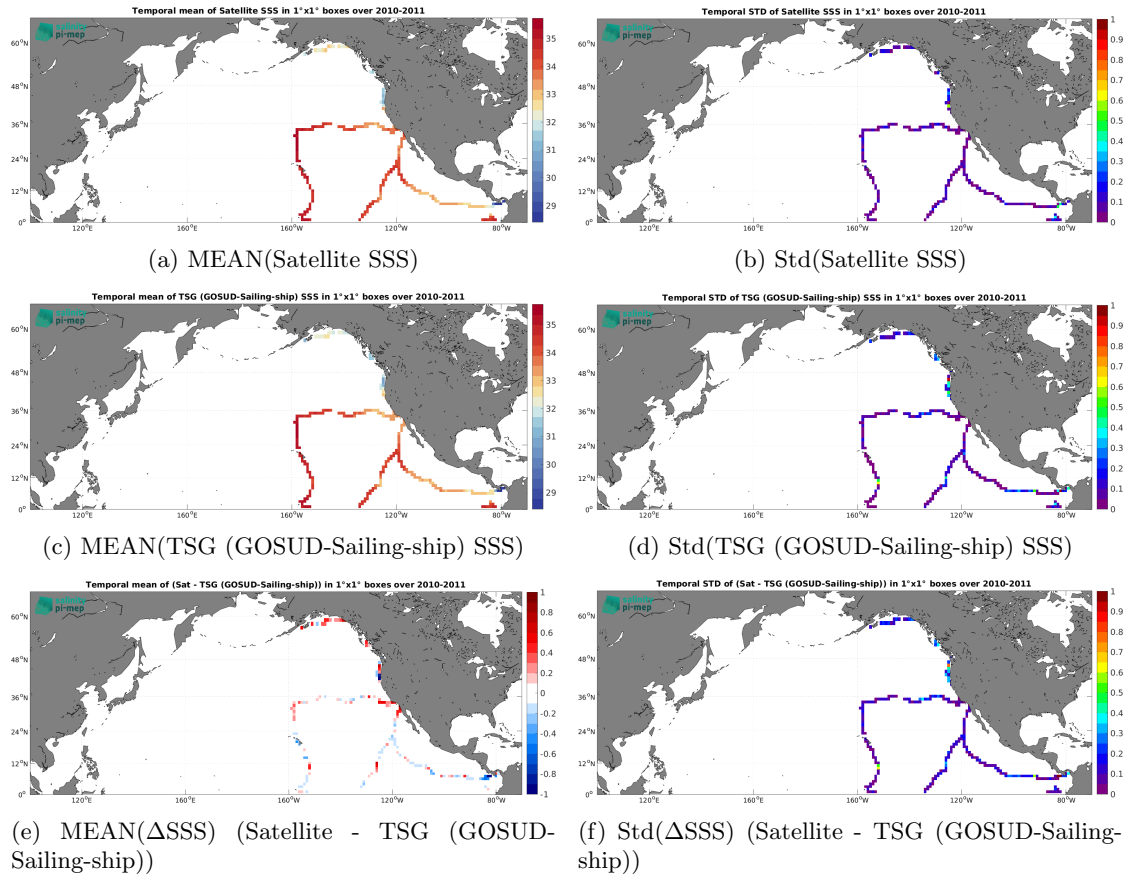
Figure 7: Temporal mean (left) and Std (right) of SSS from SMOS SSS L3 v332 - 9 Days (CATDS-CPDC) (top), TSG (GOSUD-Sailing-ship) (middle), and of \Delta SSS (Satellite - TSG (GOSUD-Sailing-ship)). Only match-up pairs are used to generate these maps.
