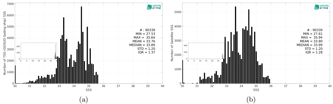
Figure 3: Histograms of SSS from TSG (GOSUD-Sailing-ship) (a) and SMOS SSS L3 v332 - 9 Days (CATDS-CPDC) (b) considering all match-up pairs per bins of 0.1 over the North Pacific Ocean Pi-MEP region and for the full satellite product period.
