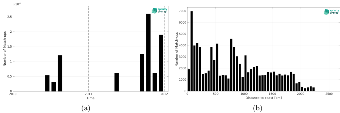
Figure 2: Number of match-ups between TSG (GOSUD-Sailing-ship) and SMOS SSS L3 v332 - 9 Days (CATDS-CPDC) SSS as a function of time (a) and as function of the distance to coast (b) over the North Pacific Ocean Pi-MEP region and for the full satellite product period.
