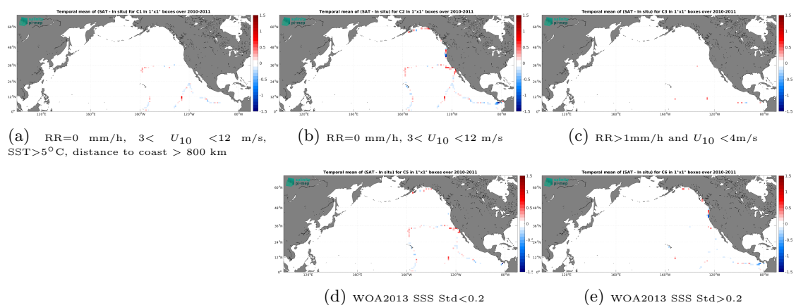
Figure 14: Temporal mean gridded over spatial boxes of size 1^\circ \times 1^\circ of \Delta SSS (SMOS SSS L3 v332 - 9 Days (CATDS-CPDC) - TSG (GOSUD-Sailing-ship)) for 5 different subdatasets corresponding to:RR=0 mm/h, 3 < U_{10} < 12 m/s, SST>5°C, distance to coast > 800 km (a), RR=0 mm/h, 3 < U_{10} < 12 m/s (b), RR>1mm/h and U_{10} < 4 m/s (c), WOA2013 SSS Std<0.2 (d), WOA2013 SSS Std>0.2 (e).
