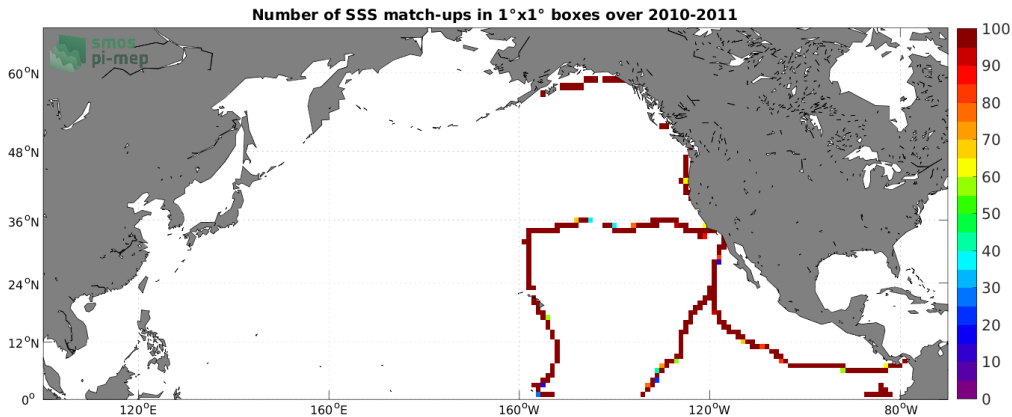
Figure 4: Number of SSS match-ups between TSG (GOSUD-Sailing-ship) SSS and the SMOS SSS L3 v332 - 9 Days (CATDS-CPDC) SSS product for the North Pacific Ocean Pi-MEP region over 1^\circ \times 1^\circ boxes and for the full satellite product period.
