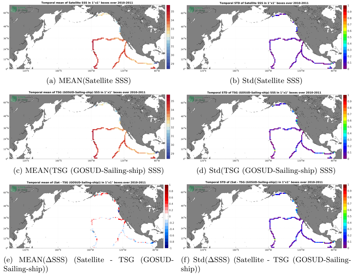
Figure 6: Temporal mean (left) and Std (right) of SSS from SMOS SSS L3 v332 - 9 Days (CATDS-CPDC) (top), TSG (GOSUD-Sailing-ship) (middle), and of \Delta SSS (Satellite - TSG (GOSUD-Sailing-ship)). Only match-up pairs are used to generate these maps.
