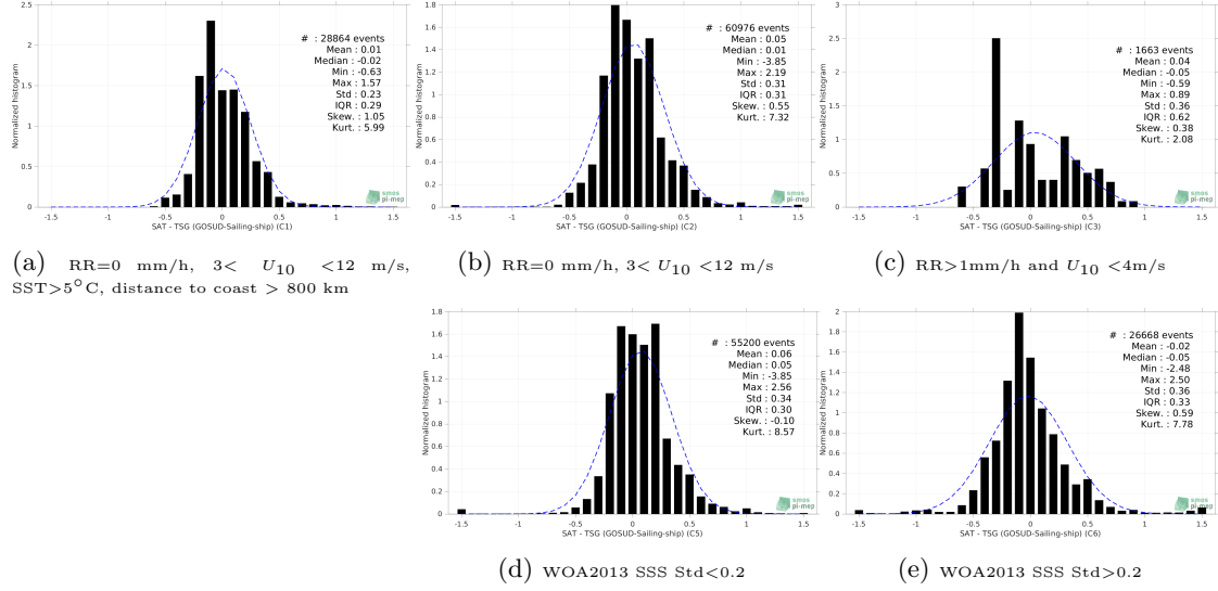
Figure 13: Normalized histogram of \Delta SSS (SMOS SSS L3 v332 - 9 Days (CATDS-CPDC) - TSG (GOSUD-Sailing-ship)) for 5 different subdatasets corresponding to: RR=0 mm/h, 3 < U_{10} < 12 m/s, SST > 5°C, distance to coast > 800 km (a), RR=0 mm/h, 3 < U_{10} < 12 m/s (b), RR > 1mm/h and U_{10} < 4 m/s (c), WOA2013 SSS Std < 0.2 (d), WOA2013 SSS Std > 0.2 (e).
