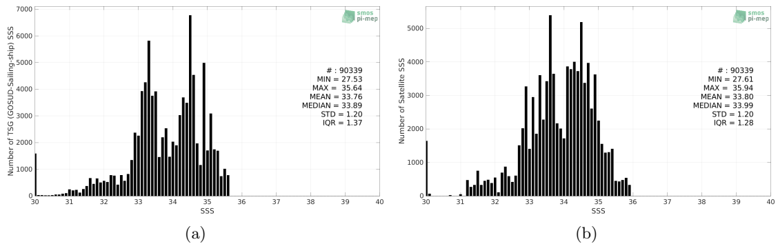
Figure 2: Histograms of SSS from TSG (GOSUD-Sailing-ship) (a) and SMOS SSS L3 v332 - 9 Days (CATDS-CPDC) (b) considering all match-up pairs per bins of 0.1 over the North Pacific Ocean Pi-MEP region and for the full satellite product period.
