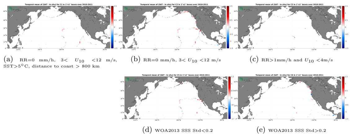
Figure 12: Temporal mean gridded over spatial boxes of size 1^\circ \times 1^\circ of \Delta SSS (SMOS SSS L3 v332 - 9 Days (CATDS-CPDC) - TSG (GOSUD-Sailing-ship)) for 5 different subdatasets corresponding to:RR=0 mm/h, 3 < U_{10} < 12 m/s, SST>5°C, distance to coast > 800 km (a), RR=0 mm/h, 3 < U_{10} < 12 m/s (b), RR>1mm/h and U_{10} < 4 m/s (c), WOA2013 SSS Std<0.2 (d), WOA2013 SSS Std>0.2 (e).
