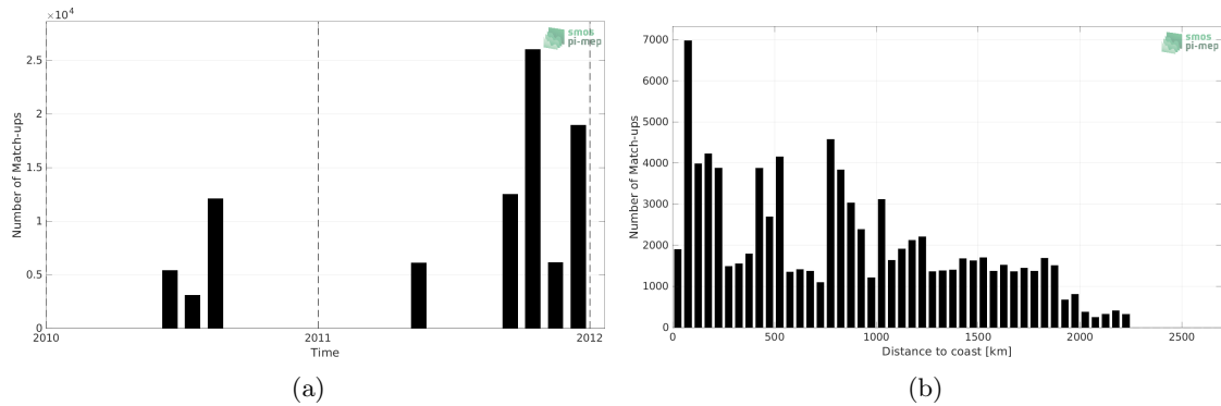
Figure 1: Number of match-ups between TSG (GOSUD-Sailing-ship) and SMOS SSS L3 v332 - 9 Days (CATDS-CPDC) SSS as a function of time (a) and as function of the distance to coast (b) over the North Pacific Ocean Pi-MEP region and for the full satellite product period.
