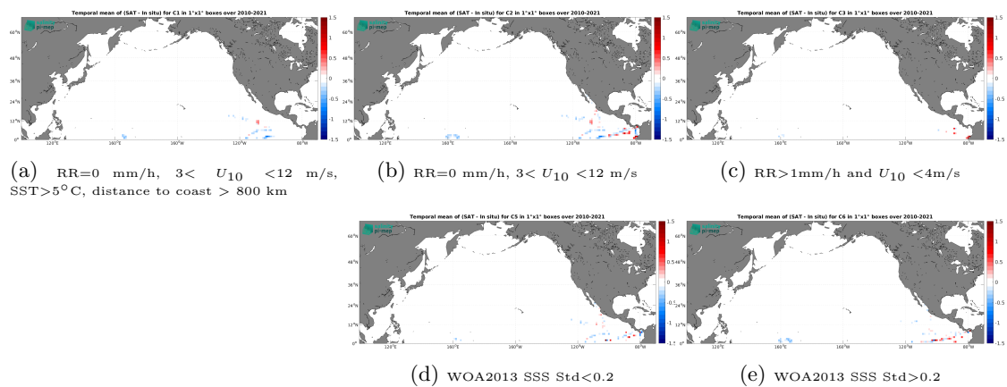
Figure 14: Temporal mean gridded over spatial boxes of size 1^\circ \times 1^\circ of \Delta\text{SSS} (SMOS SSS L3 v332 - 9 Days (CATDS-CPDC) - TSG (GOSUD-Research-vessel)) for 5 different subdatasets corresponding to: RR=0 mm/h, 3 < U_{10} < 12 m/s, SST > 5°C, distance to coast > 800 km (a), RR=0 mm/h, 3 < U_{10} < 12 m/s (b), RR > 1mm/h and U_{10} < 4 m/s (c), WOA2013 SSS Std < 0.2 (d), WOA2013 SSS Std > 0.2 (e).
