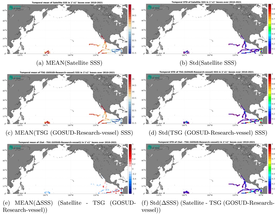
Figure 6: Temporal mean (left) and Std (right) of SSS from SMOS SSS L3 v332 - 9 Days (CATDS-CPDC) (top), TSG (GOSUD-Research-vessel) (middle), and of \Delta SSS (Satellite - TSG (GOSUD-Research-vessel)). Only match-up pairs are used to generate these maps.
