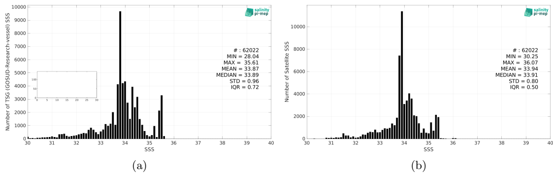
Figure 2: Histograms of SSS from TSG (GOSUD-Research-vessel) (a) and SMOS SSS L3 v332 - 9 Days (CATDS-CPDC) (b) considering all match-up pairs per bins of 0.1 over the North Pacific Ocean Pi-MEP region and for the full satellite product period.
