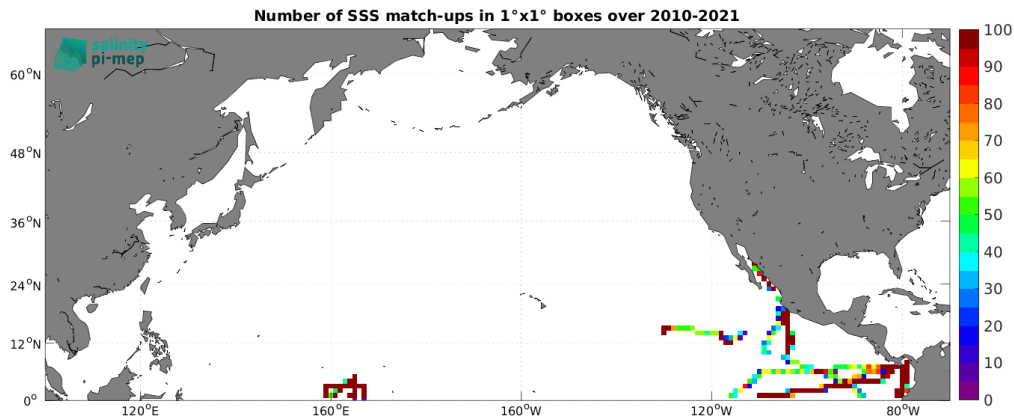
Figure 4: Number of SSS match-ups between TSG (GOSUD-Research-vessel) SSS and the SMOS SSS L3 v332 - 9 Days (CATDS-CPDC) SSS product for the North Pacific Ocean Pi-MEP region over 1^\circ \times 1^\circ boxes and for the full satellite product period.
