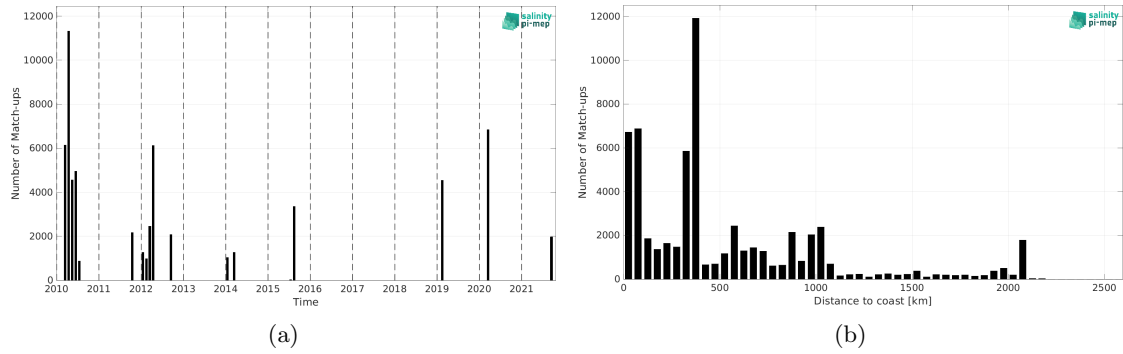
Figure 1: Number of match-ups between TSG (GOSUD-Research-vessel) and SMOS SSS L3 v332 - 9 Days (CATDS-CPDC) SSS as a function of time (a) and as function of the distance to coast (b) over the North Pacific Ocean Pi-MEP region and for the full satellite product period.
