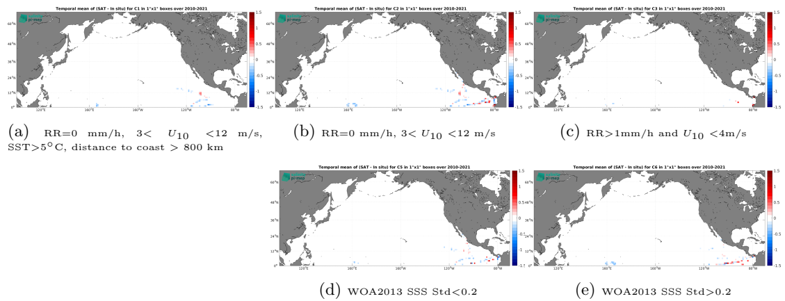
Figure 12: Temporal mean gridded over spatial boxes of size 1^\circ \times 1^\circ of \Delta SSS (SMOS SSS L3 v332 - 9 Days (CATDS-CPDC) - TSG (GOSUD-Research-vessel)) for 5 different subdatasets corresponding to: RR=0 mm/h, 3 < U_{10} < 12 m/s, SST > 5^\circ C , distance to coast > 800 km (a), RR=0 mm/h, 3 < U_{10} < 12 m/s (b), RR > 1mm/h and U_{10} < 4 m/s (c), WOA2013 SSS Std < 0.2 (d), WOA2013 SSS Std > 0.2 (e).
