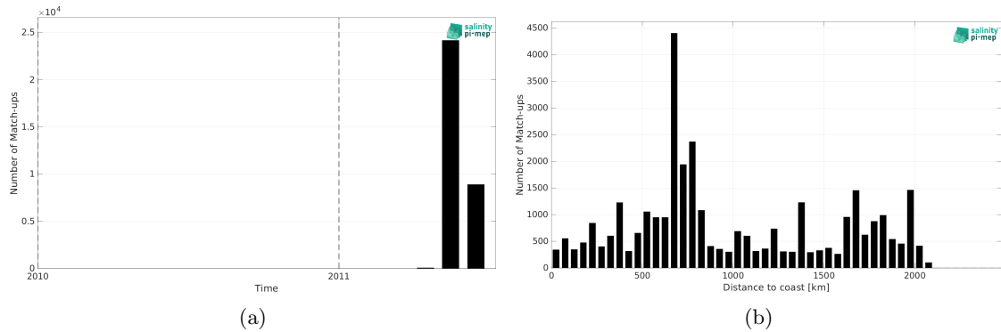
Figure 2: Number of match-ups between TSG (CSIC-UTM) and SMOS SSS L3 v332 - 9 Days (CATDS-CPDC) SSS as a function of time (a) and as function of the distance to coast (b) over the North Pacific Ocean Pi-MEP region and for the full satellite product period.
