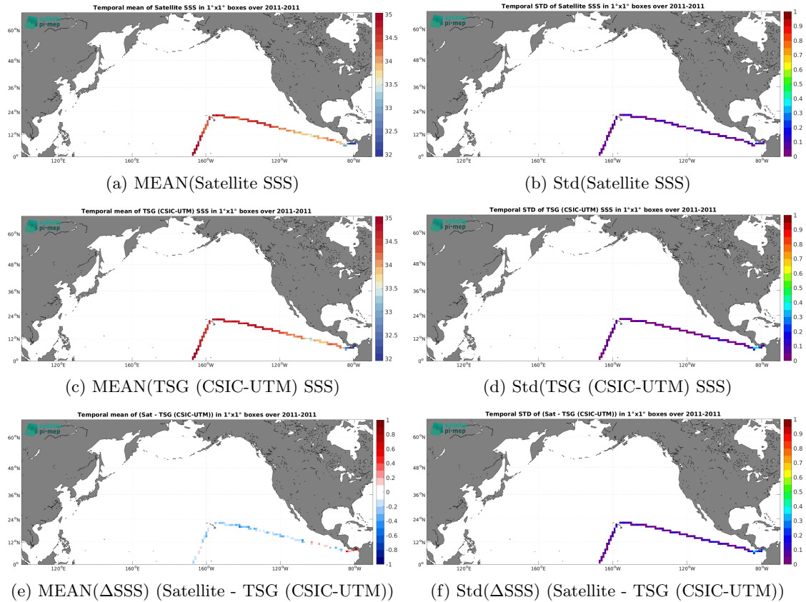
Figure 7: Temporal mean (left) and Std (right) of SSS from SMOS SSS L3 v332 - 9 Days (CATDS-CPDC) (top), TSG (CSIC-UTM) (middle), and of \Delta SSS (Satellite - TSG (CSIC-UTM)). Only match-up pairs are used to generate these maps.
