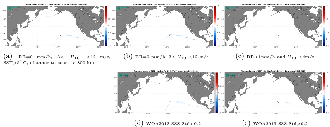
Figure 14: Temporal mean gridded over spatial boxes of size 1^\circ \times 1^\circ of \Delta\text{SSS} (SMOS SSS L3 v332 - 9 Days (CATDS-CPDC) - TSG (CSIC-UTM)) for 5 different subdatasets corresponding to:RR=0 mm/h, 3 < U_{10} < 12 m/s, SST>5°C, distance to coast > 800 km (a), RR=0 mm/h, 3 < U_{10} < 12 m/s (b), RR>1mm/h and U_{10} < 4 m/s (c), WOA2013 SSS Std<0.2 (d), WOA2013 SSS Std>0.2 (e).
