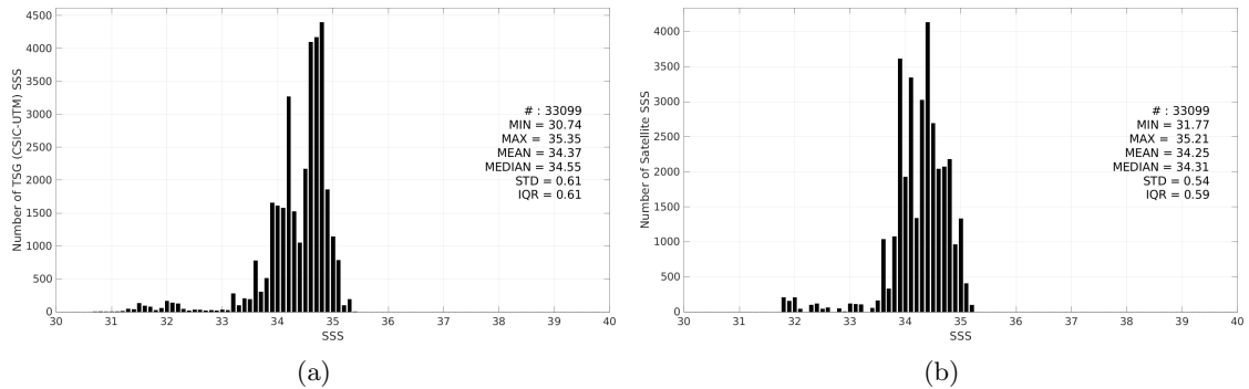
Figure 3: Histograms of SSS from TSG (CSIC-UTM) (a) and SMOS SSS L3 v332 - 9 Days (CATDS-CPDC) (b) considering all match-up pairs per bins of 0.1 over the North Pacific Ocean Pi-MEP region and for the full satellite product period.
