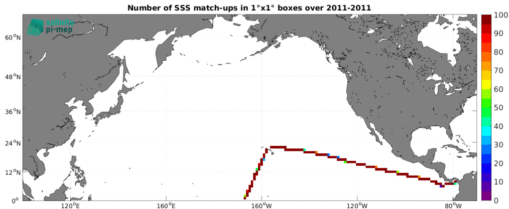
Figure 5: Number of SSS match-ups between TSG (CSIC-UTM) SSS and the SMOS SSS L3 v332 - 9 Days (CATDS-CPDC) SSS product for the North Pacific Ocean Pi-MEP region over 1^\circ \times 1^\circ boxes and for the full satellite product period.
