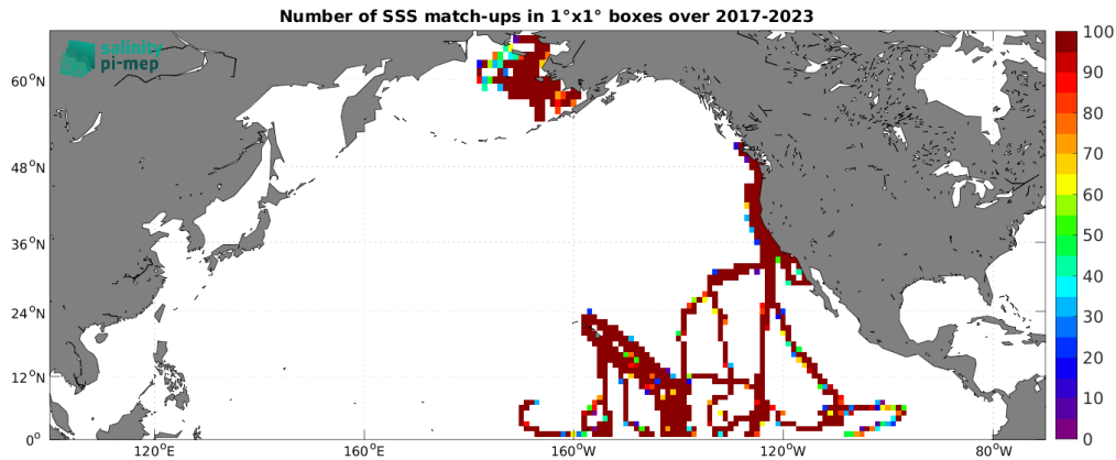
Figure 5: Number of SSS match-ups between Saildrone SSS and the SMOS SSS L3 v332 - 9 Days (CATDS-CPDC) SSS product for the North Pacific Ocean Pi-MEP region over 1^\circ \times 1^\circ boxes and for the full satellite product period.
