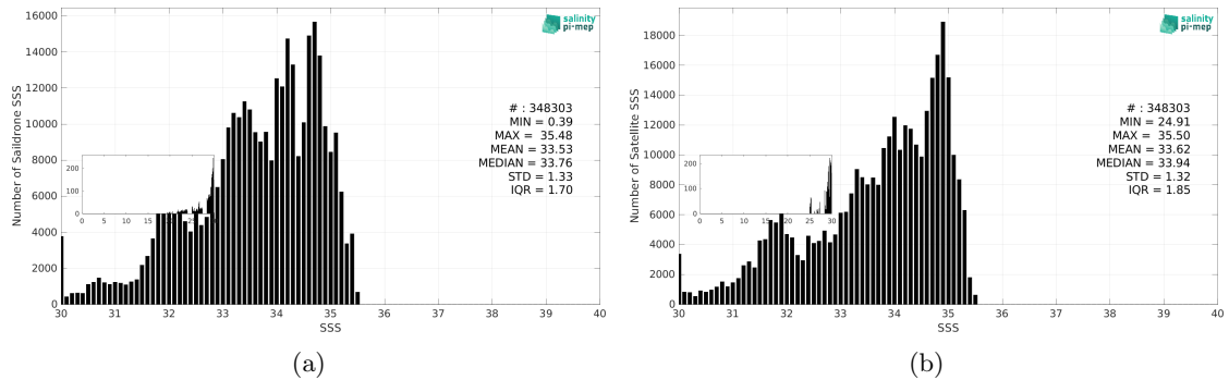
Figure 3: Histograms of SSS from Saildrone (a) and SMOS SSS L3 v332 - 9 Days (CATDS-CPDC) (b) considering all match-up pairs per bins of 0.1 over the North Pacific Ocean Pi-MEP region and for the full satellite product period.
