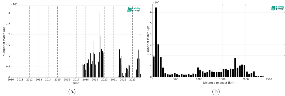
Figure 2: Number of match-ups between Saildrone and SMOS SSS L3 v332 - 9 Days (CATDS-CPDC) SSS as a function of time (a) and as function of the distance to coast (b) over the North Pacific Ocean Pi-MEP region and for the full satellite product period.
