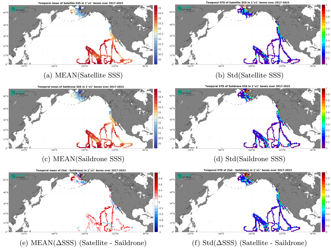
Figure 7: Temporal mean (left) and Std (right) of SSS from SMOS SSS L3 v332 - 9 Days (CATDS-CPDC) (top), Saildrone (middle), and of \Delta SSS (Satellite - Saildrone). Only match-up pairs are used to generate these maps.
