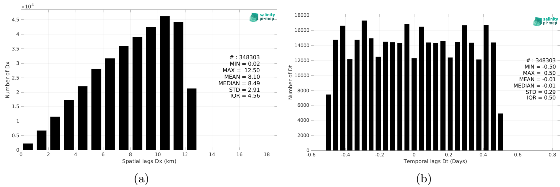
Figure 6: Histograms of the spatial (a) and temporal (b) lags between the location/time of the Sairdrone measurement and the date of the corresponding SMOS SSS L3 v332 - 9 Days (CATDS-CPDC) SSS pixel.
