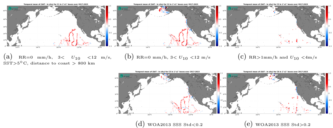
Figure 14: Temporal mean gridded over spatial boxes of size 1^\circ \times 1^\circ of \Delta SSS (SMOS SSS L3 v332 - 9 Days (CATDS-CPDC) - Sairdrone) for 5 different subdatasets corresponding to: RR=0 mm/h, 3 < U_{10} < 12 m/s, SST > 5°C, distance to coast > 800 km (a), RR=0 mm/h, 3 < U_{10} < 12 m/s (b), RR > 1mm/h and U_{10} < 4 m/s (c), WOA2013 SSS Std < 0.2 (d), WOA2013 SSS Std > 0.2 (e).
