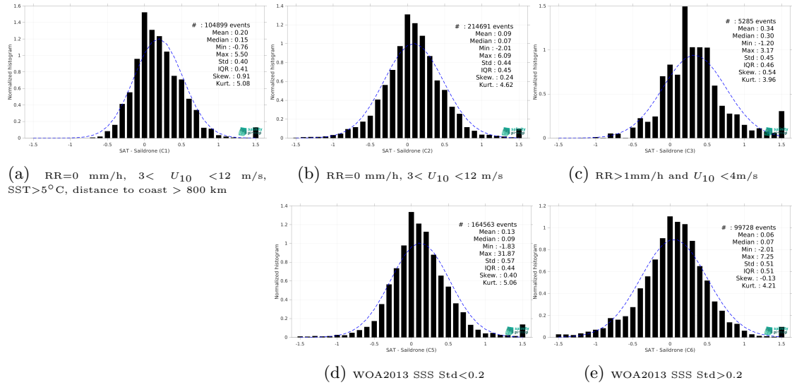
Figure 13: Normalized histogram of \Delta\text{SSS} (SMOS SSS L3 v332 - 9 Days (CATDS-CPDC) - Saildrone) for 5 different subdatasets corresponding to: RR=0 mm/h, 3 < U_{10} < 12 m/s, SST>5°C, distance to coast > 800 km (a), RR=0 mm/h, 3 < U_{10} < 12 m/s (b), RR>1mm/h and U_{10} < 4 m/s (c), WOA2013 SSS Std<0.2 (d), WOA2013 SSS Std>0.2 (e).
