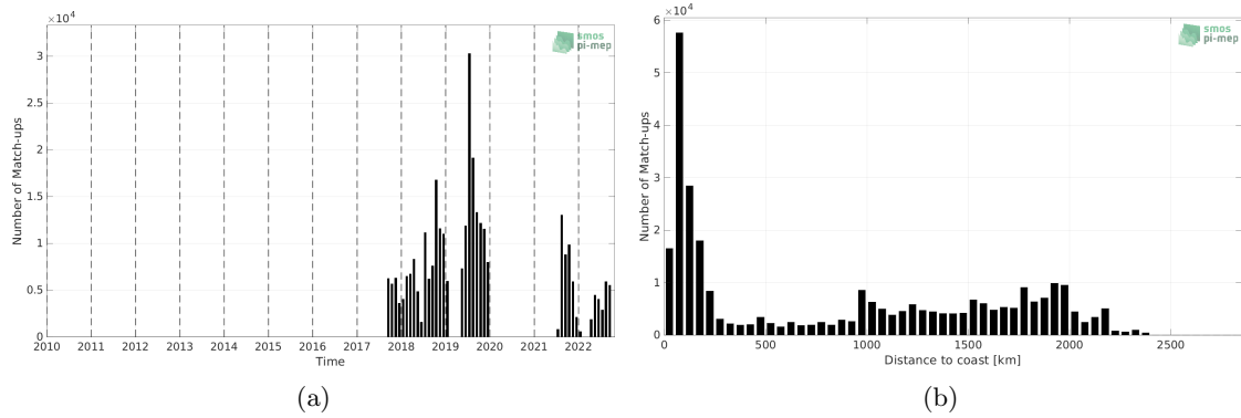
Figure 1: Number of match-ups between Saildrone and SMOS SSS L3 v332 - 9 Days (CATDS-CPDC) SSS as a function of time (a) and as function of the distance to coast (b) over the North Pacific Ocean Pi-MEP region and for the full satellite product period.
