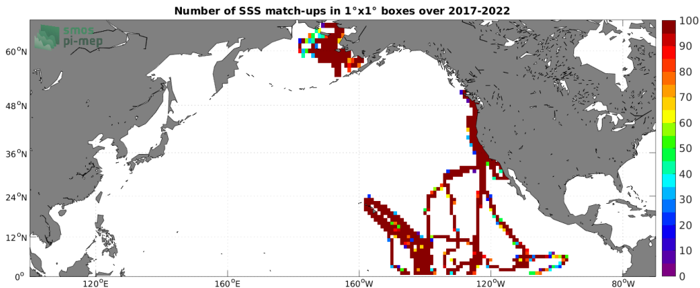
Figure 4: Number of SSS match-ups between Saildrone SSS and the SMOS SSS L3 v332 - 9 Days (CATDS-CPDC) SSS product for the North Pacific Ocean Pi-MEP region over 1^\circ \times 1^\circ boxes and for the full satellite product period.
