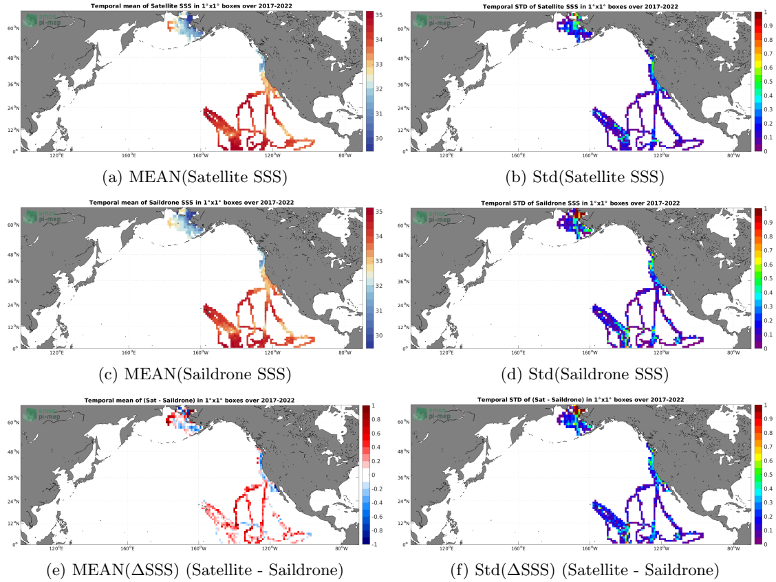
Figure 6: Temporal mean (left) and Std (right) of SSS from SMOS SSS L3 v332 - 9 Days (CATDS-CPDC) (top), Saildrone (middle), and of \Delta SSS (Satellite - Saildrone). Only match-up pairs are used to generate these maps.
