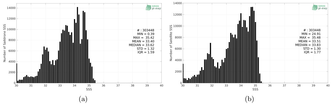
Figure 2: Histograms of SSS from Saildrone (a) and SMOS SSS L3 v332 - 9 Days (CATDS-CPDC) (b) considering all match-up pairs per bins of 0.1 over the North Pacific Ocean Pi-MEP region and for the full satellite product period.
