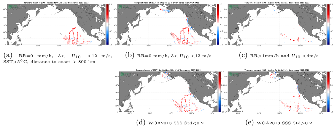
Figure 12: Temporal mean gridded over spatial boxes of size 1^\circ \times 1^\circ of \Delta SSS (SMOS SSS L3 v332 - 9 Days (CATDS-CPDC) - Saildrone) for 5 different subdatasets corresponding to:RR=0 mm/h, 3 < U_{10} < 12 m/s, SST > 5^\circ C , distance to coast > 800 km (a), RR=0 mm/h, 3 < U_{10} < 12 m/s (b), RR>1mm/h and U_{10} < 4 m/s (c), WOA2013 SSS Std<0.2 (d), WOA2013 SSS Std>0.2 (e).
