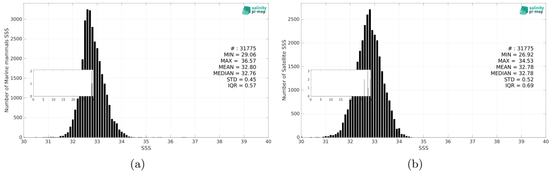
Figure 3: Histograms of SSS from Marine mammals (a) and SMOS SSS L3 v332 - 9 Days (CATDS-CPDC) (b) considering all match-up pairs per bins of 0.1 over the North Pacific Ocean Pi-MEP region and for the full satellite product period.
