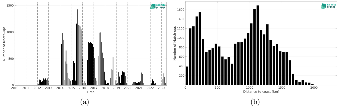
Figure 2: Number of match-ups between Marine mammals and SMOS SSS L3 v332 - 9 Days (CATDS-CPDC) SSS as a function of time (a) and as function of the distance to coast (b) over the North Pacific Ocean Pi-MEP region and for the full satellite product period.
