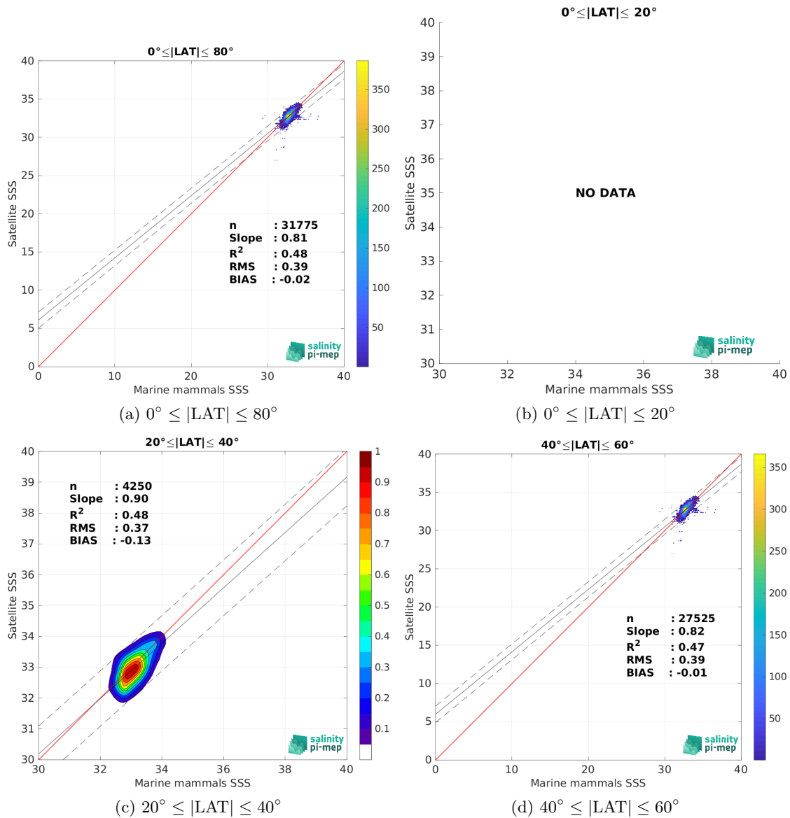
Figure 10: Contour maps of the concentration of SMOS SSS L3 v332 - 9 Days (CATDS-CPDC) SSS (y-axis) versus Marine mammals SSS (x-axis) at match-up pairs for different latitude bands. For each plot, the red line shows x=y . The black thin and dashed lines indicate a linear fit through the data cloud and the \pm 95\% confidence levels, respectively. The number match-up pairs n , the slope and R^2 coefficient of the linear fit, the root mean square (RMS) and the mean bias between satellite and in situ data are indicated for each latitude band in each plots.
