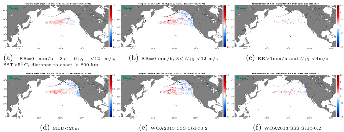
Figure 14: Temporal mean gridded over spatial boxes of size 1^\circ \times 1^\circ of \Delta SSS (SMOS SSS L3 v332 - 9 Days (CATDS-CPDC) - Marine mammals) for 6 different subdatasets corresponding to:RR=0 mm/h, 3 < U_{10} < 12 m/s, SST>5°C, distance to coast > 800 km (a), RR=0 mm/h, 3 < U_{10} < 12 m/s (b), RR>1mm/h and U_{10} < 4 m/s (c),MLD<20m (d),WOA2013 SSS Std<0.2 (e),WOA2013 SSS Std>0.2 (f).
