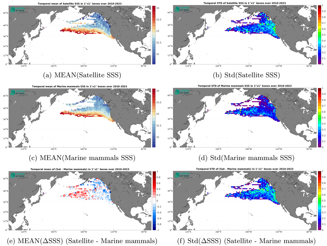
Figure 7: Temporal mean (left) and Std (right) of SSS from SMOS SSS L3 v332 - 9 Days (CATDS-CPDC) (top), Marine mammals (middle), and of \Delta SSS (Satellite - Marine mammals). Only match-up pairs are used to generate these maps.
