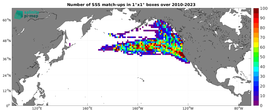
Figure 5: Number of SSS match-ups between Marine mammals SSS and the SMOS SSS L3 v332 - 9 Days (CATDS-CPDC) SSS product for the North Pacific Ocean Pi-MEP region over 1^\circ \times 1^\circ boxes and for the full satellite product period.
