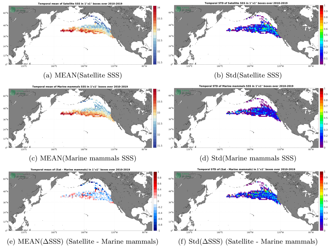
Figure 6: Temporal mean (left) and Std (right) of SSS from SMOS SSS L3 v332 - 9 Days (CATDS-CPDC) (top), Marine mammals (middle), and of \Delta SSS (Satellite - Marine mammals). Only match-up pairs are used to generate these maps.
