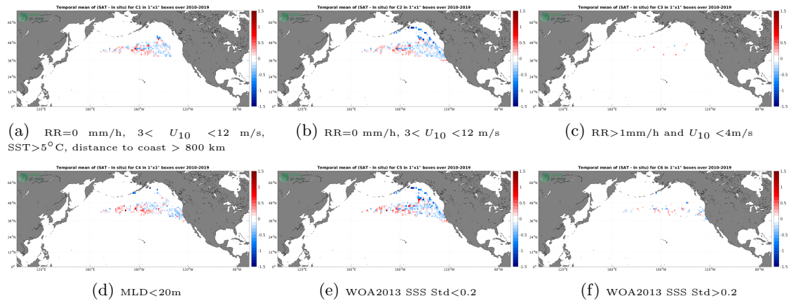
Figure 12: Temporal mean gridded over spatial boxes of size 1^\circ \times 1^\circ of \Delta SSS (SMOS SSS L3 v332 - 9 Days (CATDS-CPDC) - Marine mammals) for 6 different subdatasets corresponding to:RR=0 mm/h, 3 < U_{10} < 12 m/s, SST >5^\circ C, distance to coast > 800 km (a), RR=0 mm/h, 3 < U_{10} < 12 m/s (b), RR >1 mm/h and U_{10} < 4 m/s (c),MLD <20 m (d),WOA2013 SSS Std <0.2 (e),WOA2013 SSS Std >0.2 (f).
