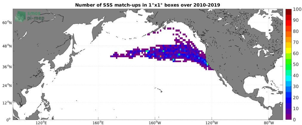
Figure 4: Number of SSS match-ups between Marine mammals SSS and the SMOS SSS L3 v332 - 9 Days (CATDS-CPDC) SSS product for the North Pacific Ocean Pi-MEP region over 1^\circ \times 1^\circ boxes and for the full satellite product period.
