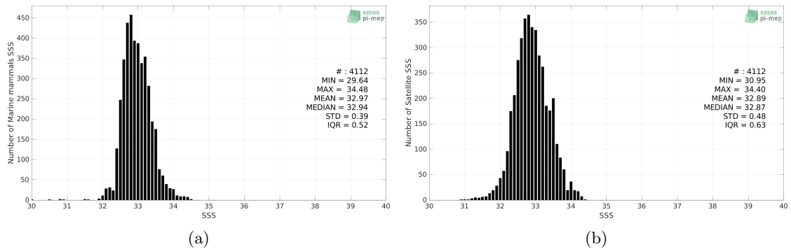
Figure 2: Histograms of SSS from Marine mammals (a) and SMOS SSS L3 v332 - 9 Days (CATDS-CPDC) (b) considering all match-up pairs per bins of 0.1 over the North Pacific Ocean Pi-MEP region and for the full satellite product period.
