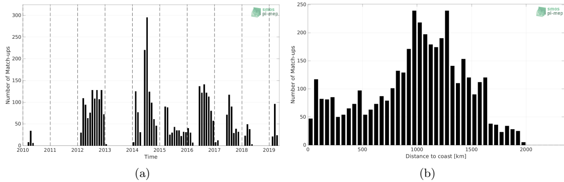
Figure 1: Number of match-ups between Marine mammals and SMOS SSS L3 v332 - 9 Days (CATDS-CPDC) SSS as a function of time (a) and as function of the distance to coast (b) over the North Pacific Ocean Pi-MEP region and for the full satellite product period.
