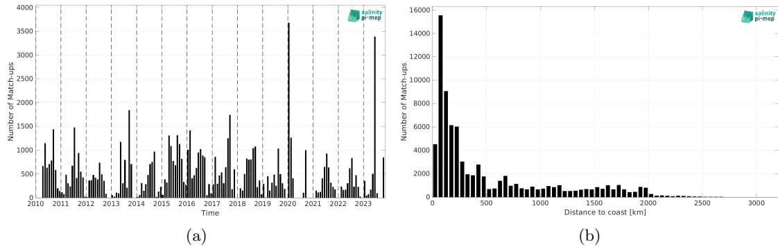
Figure 1: Number of match-ups between TSG (SAMOS) and SMOS SSS L2Q v331 - 0.25 Deg (CATDS-CPDC) SSS as a function of time (a) and as function of the distance to coast (b) over the North Pacific Ocean Pi-MEP region and for the full satellite product period.
