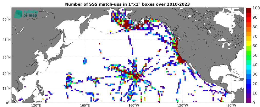
Figure 4: Number of SSS match-ups between TSG (SAMOS) SSS and the SMOS SSS L2Q v331 - 0.25 Deg (CATDS-CPDC) SSS product for the North Pacific Ocean Pi-MEP region over 1^\circ \times 1^\circ boxes and for the full satellite product period.
