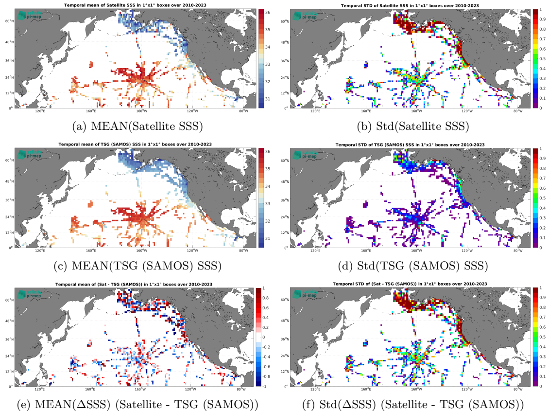
Figure 6: Temporal mean (left) and Std (right) of SSS from SMOS SSS L2Q v331 - 0.25 Deg (CATDS-CPDC) (top), TSG (SAMOS) (middle), and of \Delta SSS (Satellite - TSG (SAMOS)). Only match-up pairs are used to generate these maps.
